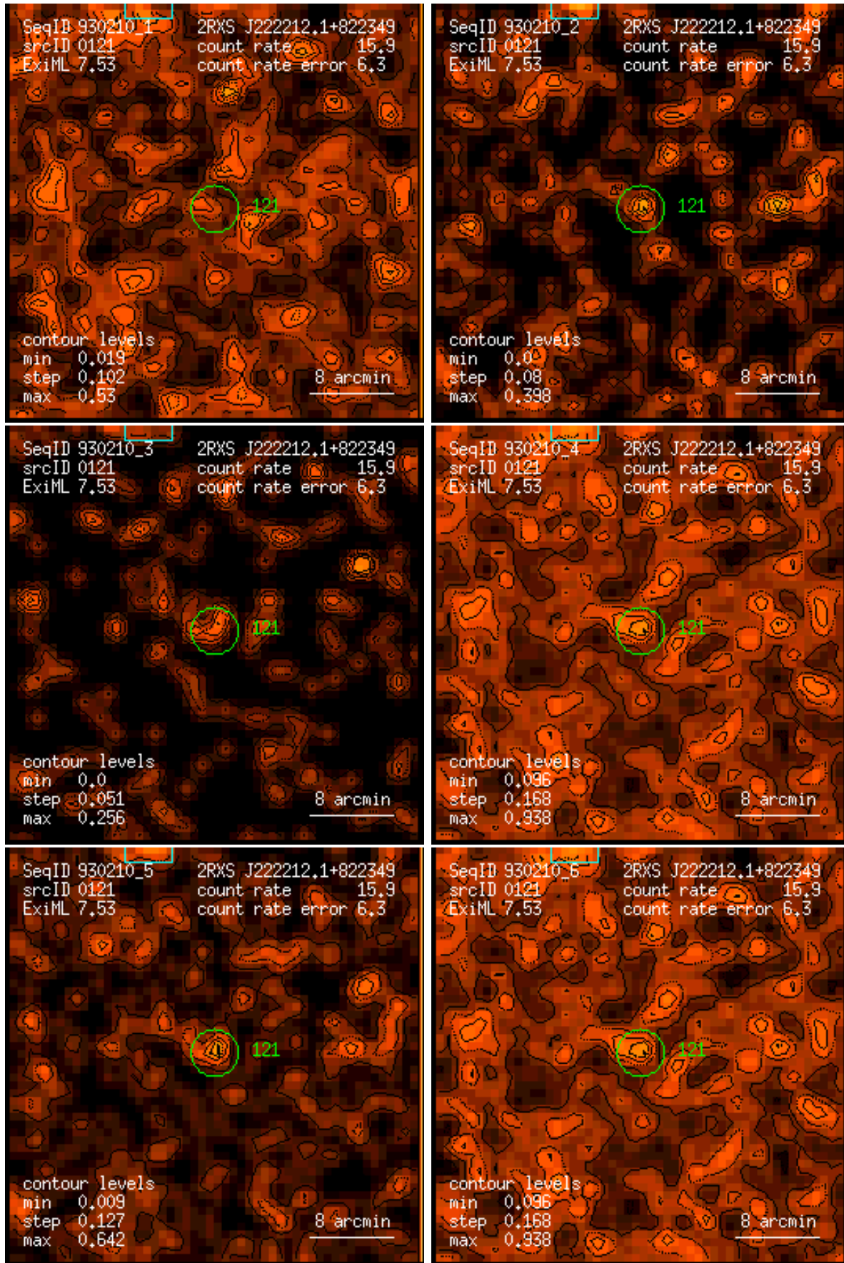
Figure 121: RASS 930210: detection 0121: band rate images, Gaussian filter: (1) PSPC channels 11 – 41, (2) 52 – 90, (3) 91 – 201, (4) 11 – 235, (5) 52 – 201, (6) 11 – 201. Broad band rates in counts/ks. Band rate contour levels in counts/ks/arcmin 2 .
