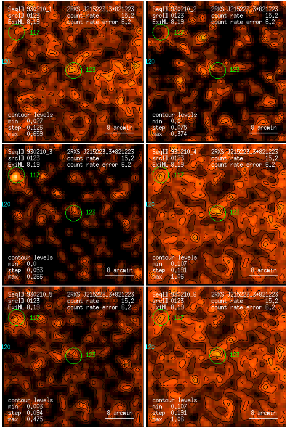
Figure 123: RASS 930210: detection 0123: band rate images, Gaussian filter: (1) PSPC channels 11 – 41, (2) 52 – 90, (3) 91 – 201, (4) 11 – 235, (5) 52 – 201, (6) 11 – 201. Broad band rates in counts/ks. Band rate contour levels in counts/ks/arcmin 2 .
