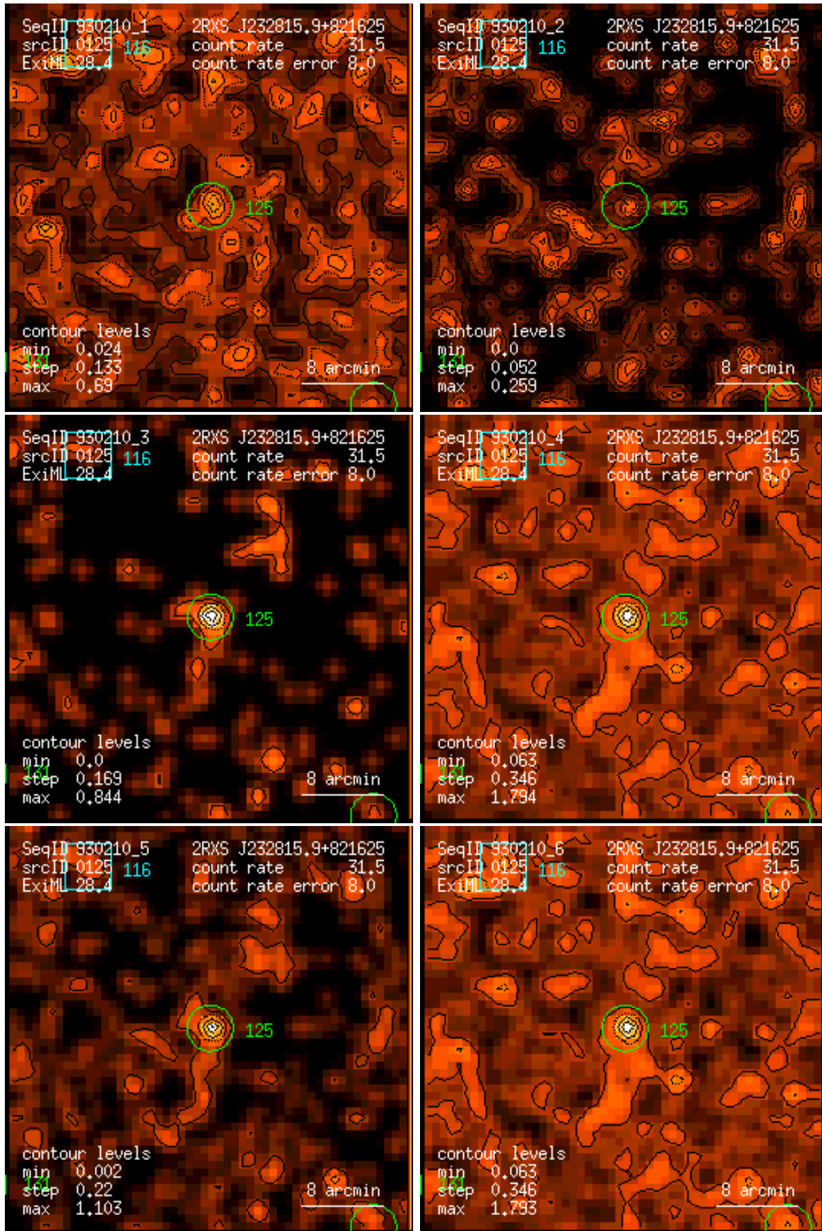
Figure 125: RASS 930210: detection 0125: band rate images, Gaussian filter: (1) PSPC channels 11 – 41, (2) 52 – 90, (3) 91 – 201, (4) 11 – 235, (5) 52 – 201, (6) 11 – 201. Broad band rates in counts/ks. Band rate contour levels in counts/ks/arcmin 2 .
