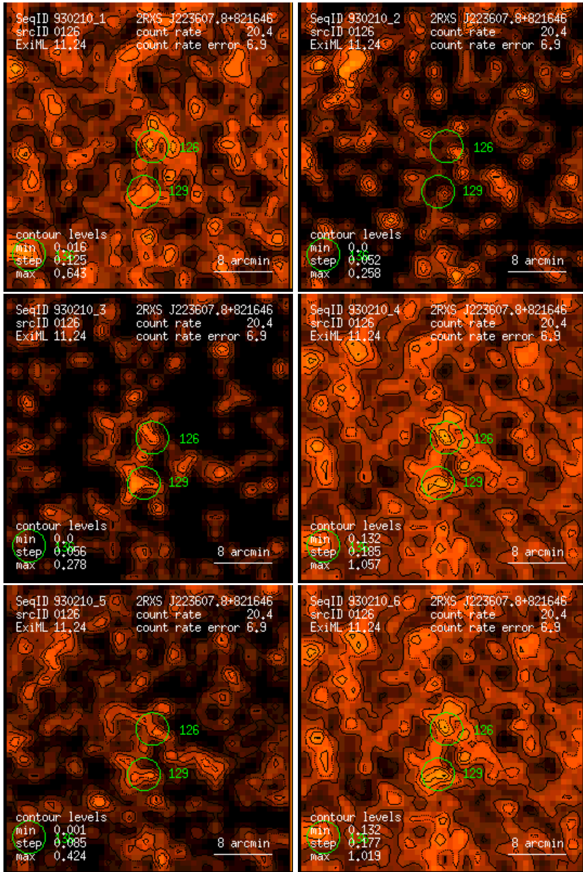
Figure 126: RASS 930210: detection 0126: band rate images, Gaussian filter: (1) PSPC channels 11 – 41, (2) 52 – 90, (3) 91 – 201, (4) 11 – 235, (5) 52 – 201, (6) 11 – 201. Broad band rates in counts/ks. Band rate contour levels in counts/ks/arcmin 2 .
