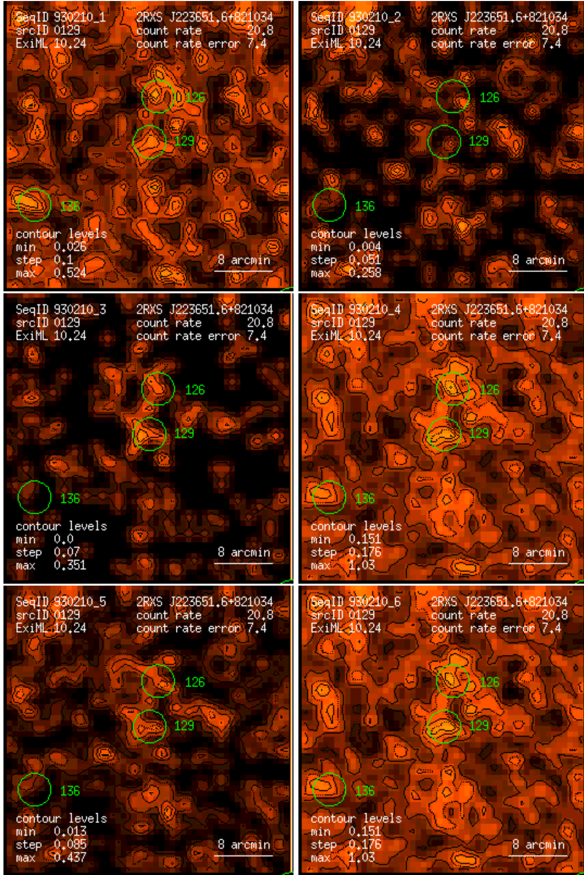
Figure 129: RASS 930210: detection 0129: band rate images, Gaussian filter: (1) PSPC channels 11 – 41, (2) 52 – 90, (3) 91 – 201, (4) 11 – 235, (5) 52 – 201, (6) 11 – 201. Broad band rates in counts/ks. Band rate contour levels in counts/ks/arcmin 2 .
