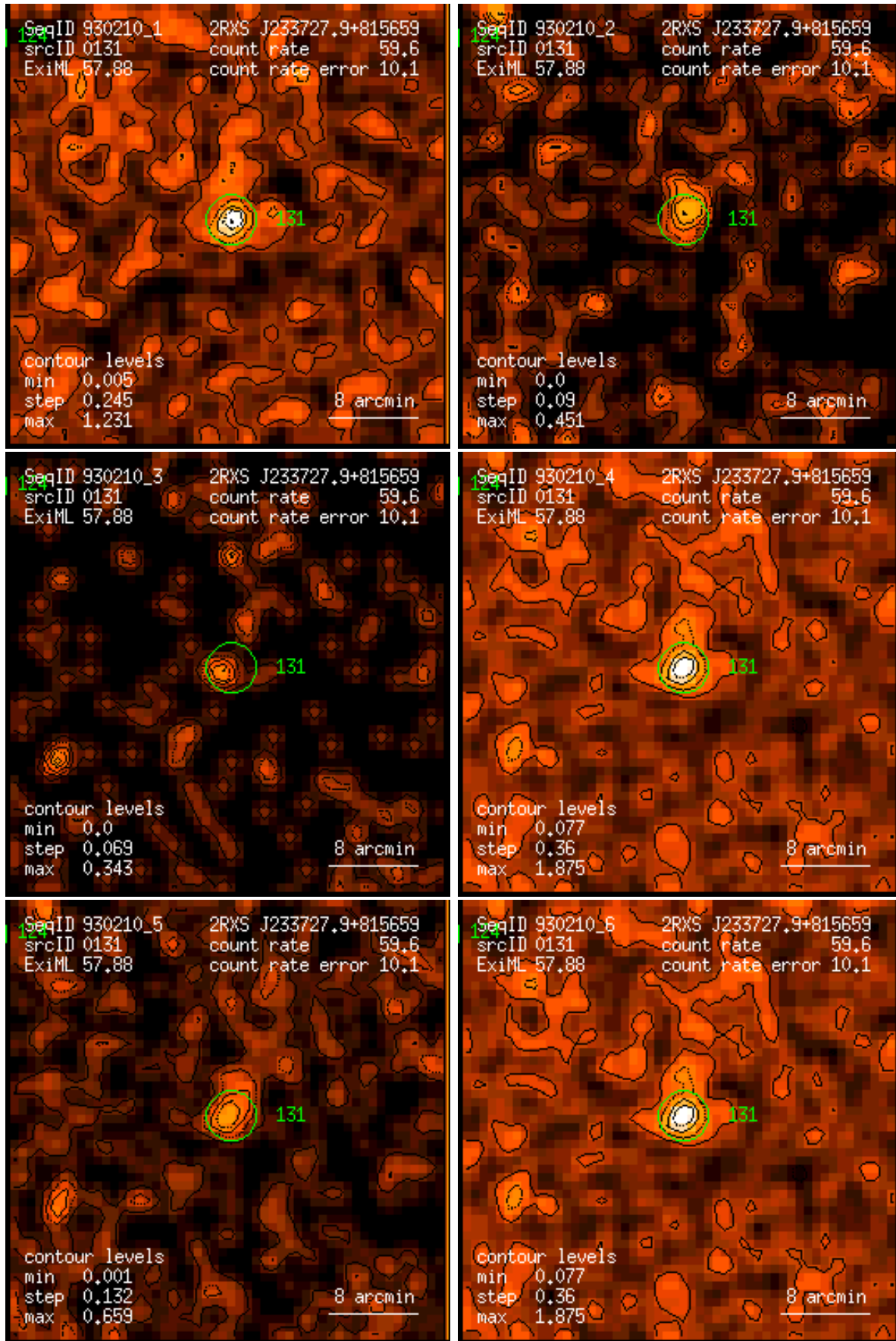
Figure 131: RASS 930210: detection 0131: band rate images, Gaussian filter: (1) PSPC channels 11 – 41, (2) 52 – 90, (3) 91 – 201, (4) 11 – 235, (5) 52 – 201, (6) 11 – 201. Broad band rates in counts/ks. Band rate contour levels in counts/ks/arcmin 2 .
