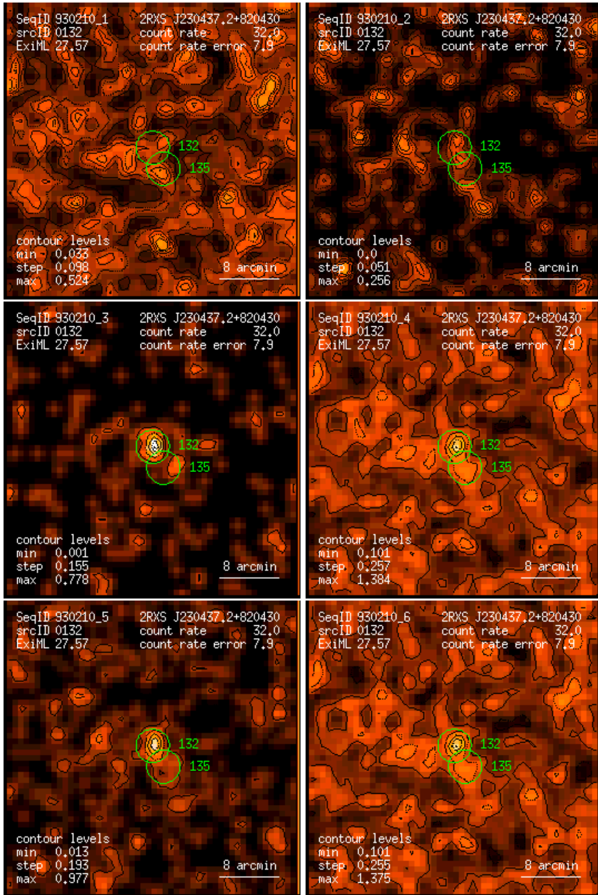
Figure 132: RASS 930210: detection 0132: band rate images, Gaussian filter: (1) PSPC channels 11 – 41, (2) 52 – 90, (3) 91 – 201, (4) 11 – 235, (5) 52 – 201, (6) 11 – 201. Broad band rates in counts/ks. Band rate contour levels in counts/ks/arcmin 2 .
