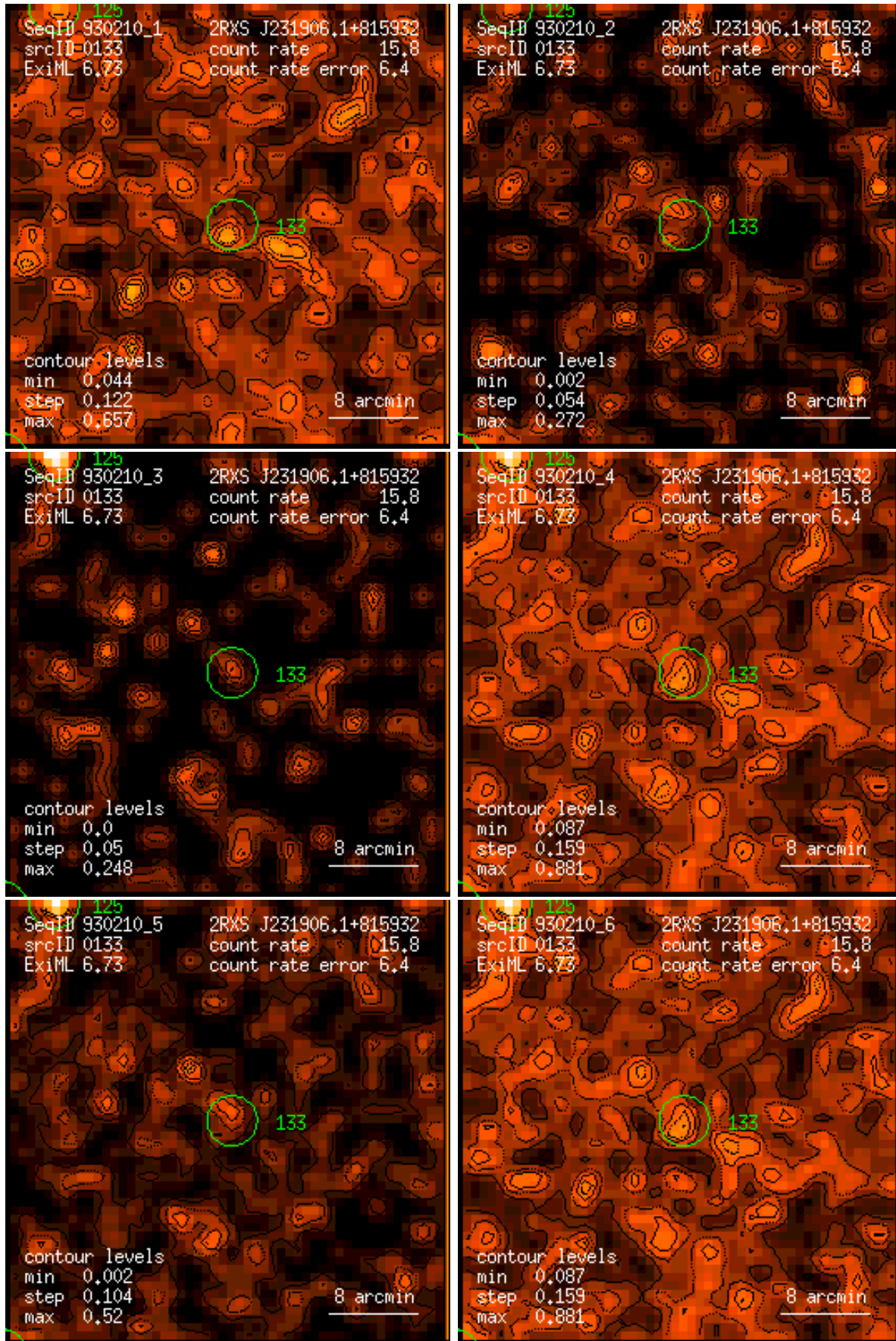
Figure 133: RASS 930210: detection 0133: band rate images, Gaussian filter: (1) PSPC channels 11 – 41, (2) 52 – 90, (3) 91 – 201, (4) 11 – 235, (5) 52 – 201, (6) 11 – 201. Broad band rates in counts/ks. Band rate contour levels in counts/ks/arcmin 2 .
