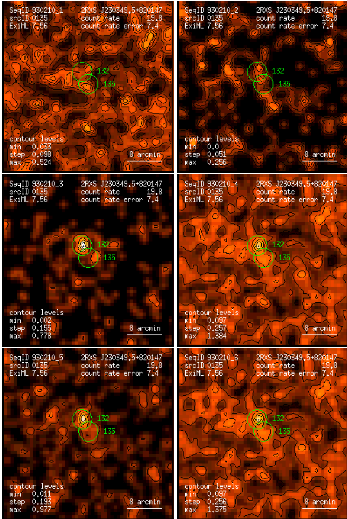
Figure 135: RASS 930210: detection 0135: band rate images, Gaussian filter: (1) PSPC channels 11 – 41, (2) 52 – 90, (3) 91 – 201, (4) 11 – 235, (5) 52 – 201, (6) 11 – 201. Broad band rates in counts/ks. Band rate contour levels in counts/ks/arcmin 2 .
