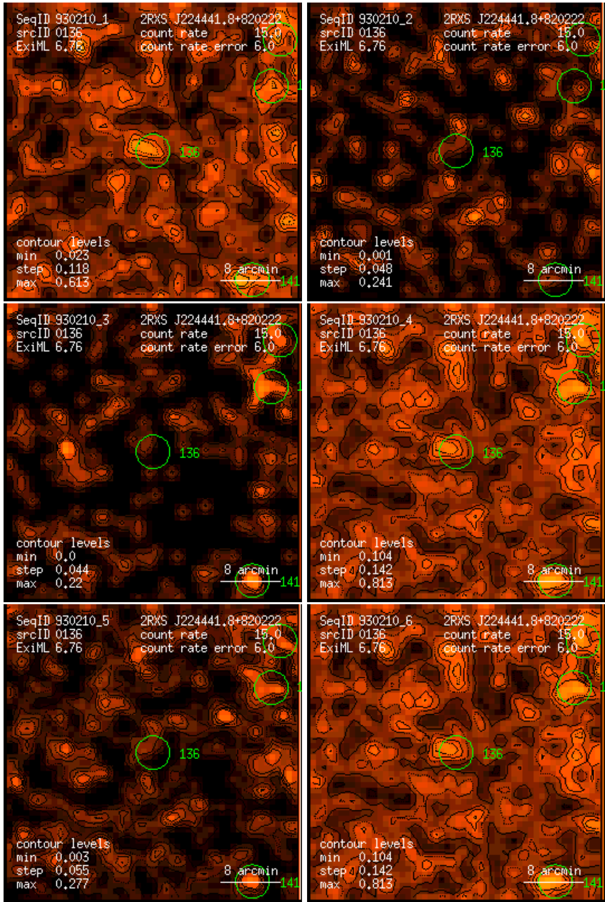
Figure 136: RASS 930210: detection 0136: band rate images, Gaussian filter: (1) PSPC channels 11 – 41, (2) 52 – 90, (3) 91 – 201, (4) 11 – 235, (5) 52 – 201, (6) 11 – 201. Broad band rates in counts/ks. Band rate contour levels in counts/ks/arcmin 2 .
