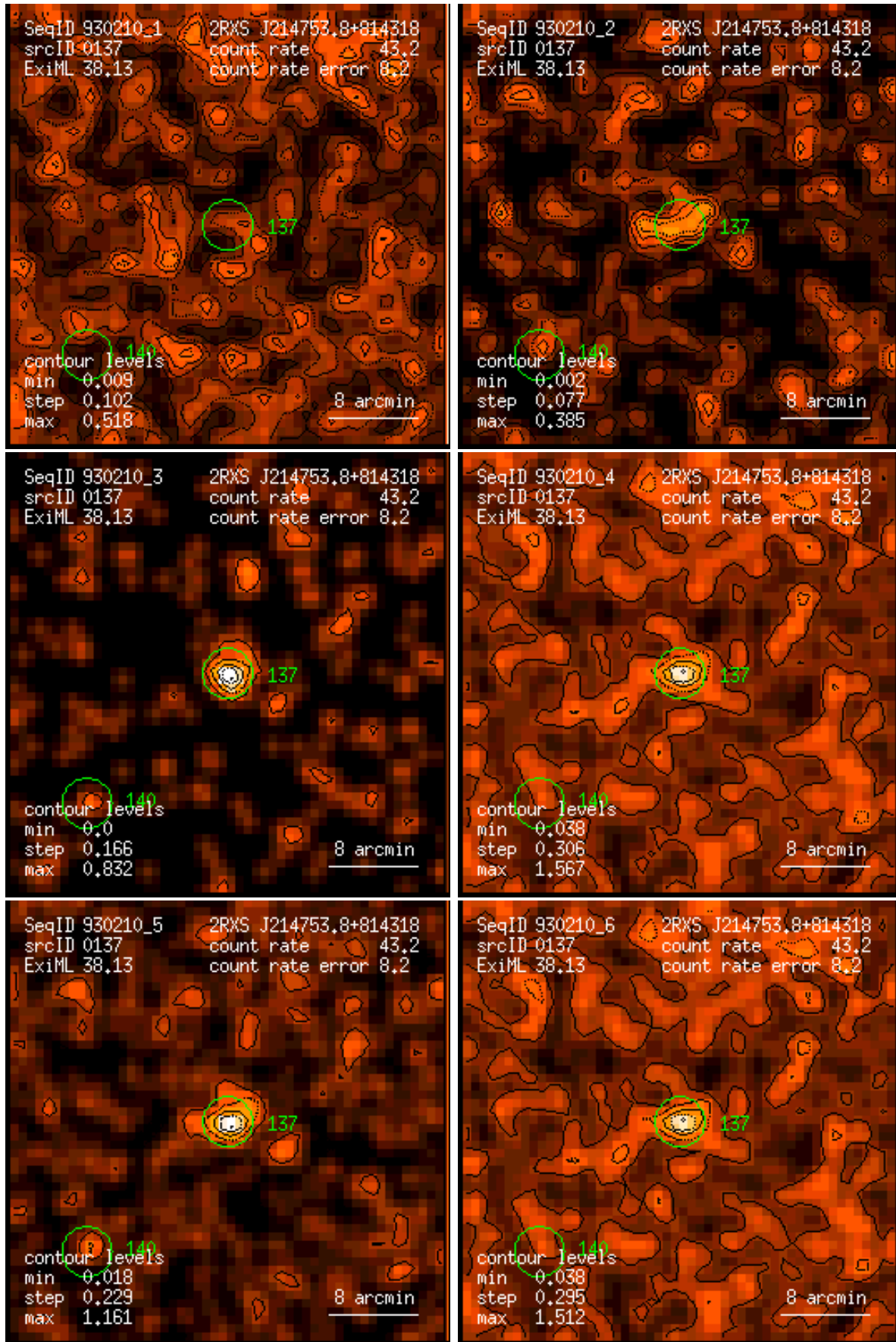
Figure 137: RASS 930210: detection 0137: band rate images, Gaussian filter: (1) PSPC channels 11 – 41, (2) 52 – 90, (3) 91 – 201, (4) 11 – 235, (5) 52 – 201, (6) 11 – 201. Broad band rates in counts/ks. Band rate contour levels in counts/ks/arcmin 2 .
