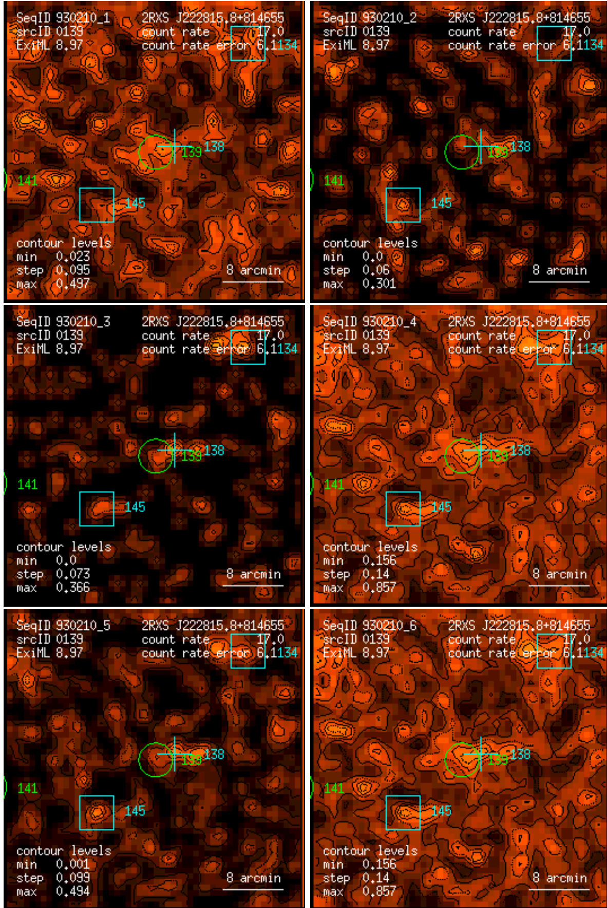
Figure 139: RASS 930210: detection 0139: band rate images, Gaussian filter: (1) PSPC channels 11 – 41, (2) 52 – 90, (3) 91 – 201, (4) 11 – 235, (5) 52 – 201, (6) 11 – 201. Broad band rates in counts/ks. Band rate contour levels in counts/ks/arcmin 2 .
