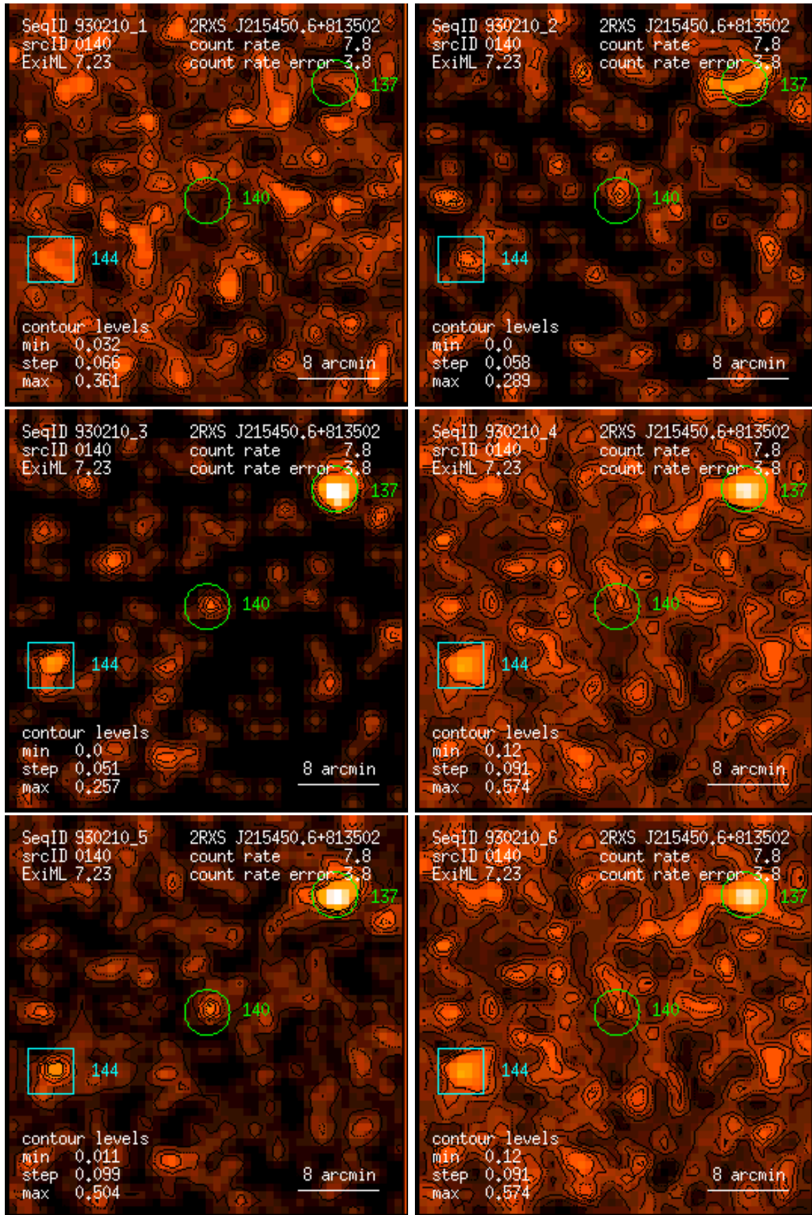
Figure 140: RASS 930210: detection 0140: band rate images, Gaussian filter: (1) PSPC channels 11 – 41, (2) 52 – 90, (3) 91 – 201, (4) 11 – 235, (5) 52 – 201, (6) 11 – 201. Broad band rates in counts/ks. Band rate contour levels in counts/ks/arcmin 2 .
