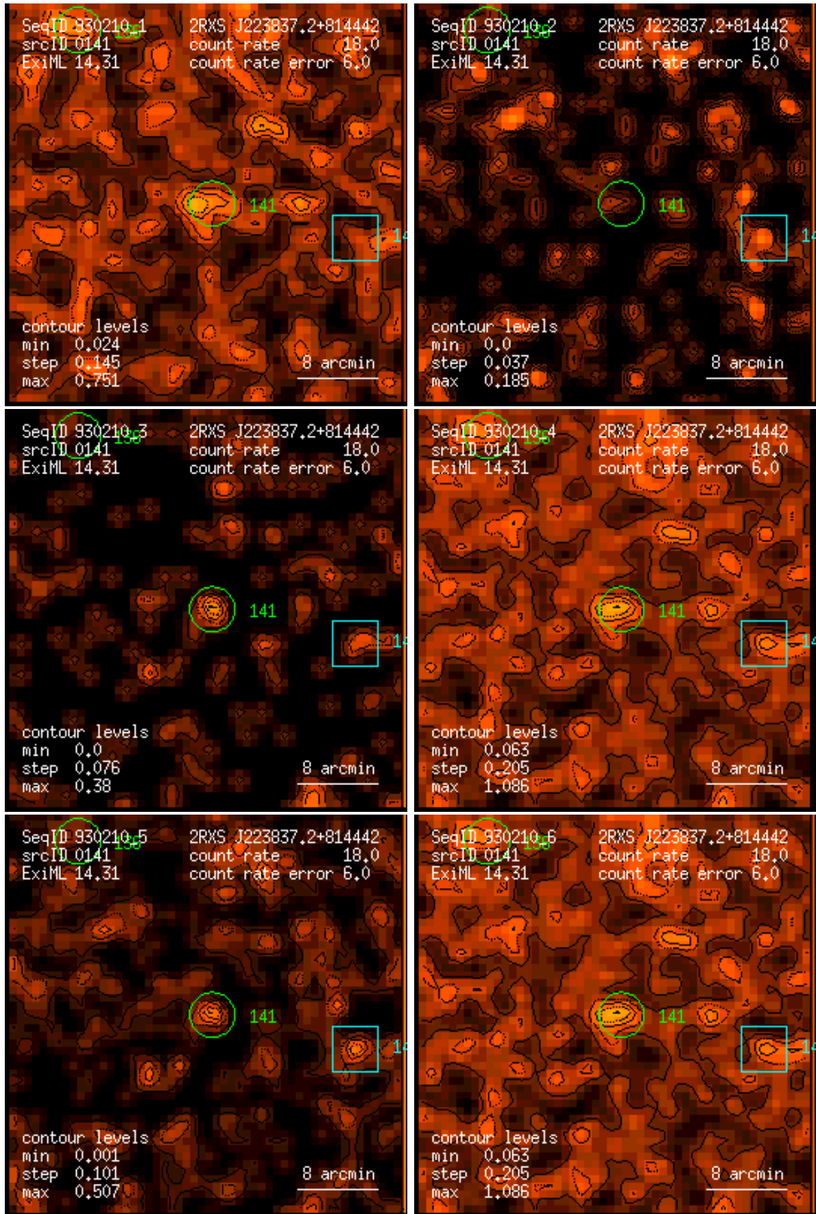
Figure 141: RASS 930210: detection 0141: band rate images, Gaussian filter: (1) PSPC channels 11 – 41, (2) 52 – 90, (3) 91 – 201, (4) 11 – 235, (5) 52 – 201, (6) 11 – 201. Broad band rates in counts/ks. Band rate contour levels in counts/ks/arcmin 2 .
