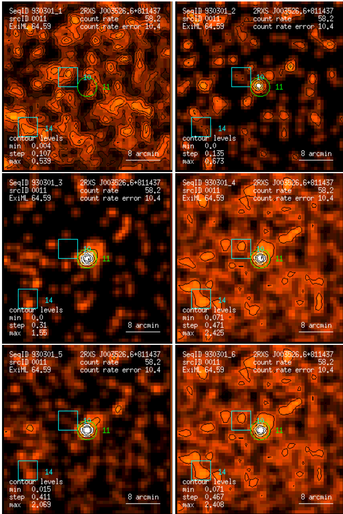
Figure 11: RASS 930301: detection 0011: band rate images, Gaussian filter: (1) PSPC channels 11 – 41, (2) 52 – 90, (3) 91 – 201, (4) 11 – 235, (5) 52 – 201, (6) 11 – 201. Broad band rates in counts/ks. Band rate contour levels in counts/ks/arcmin 2 .
