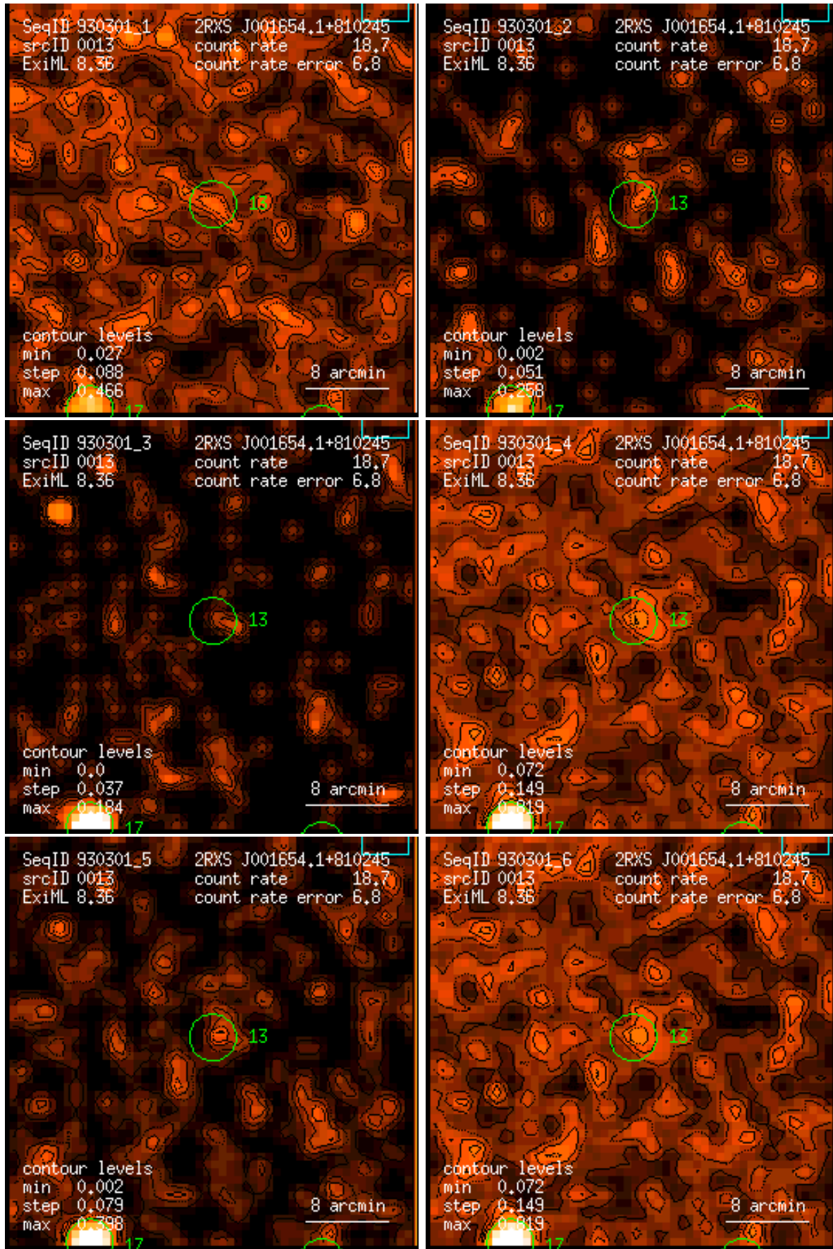
Figure 13: RASS 930301: detection 0013: band rate images, Gaussian filter: (1) PSPC channels 11 – 41, (2) 52 – 90, (3) 91 – 201, (4) 11 – 235, (5) 52 – 201, (6) 11 – 201. Broad band rates in counts/ks. Band rate contour levels in counts/ks/arcmin 2 .
