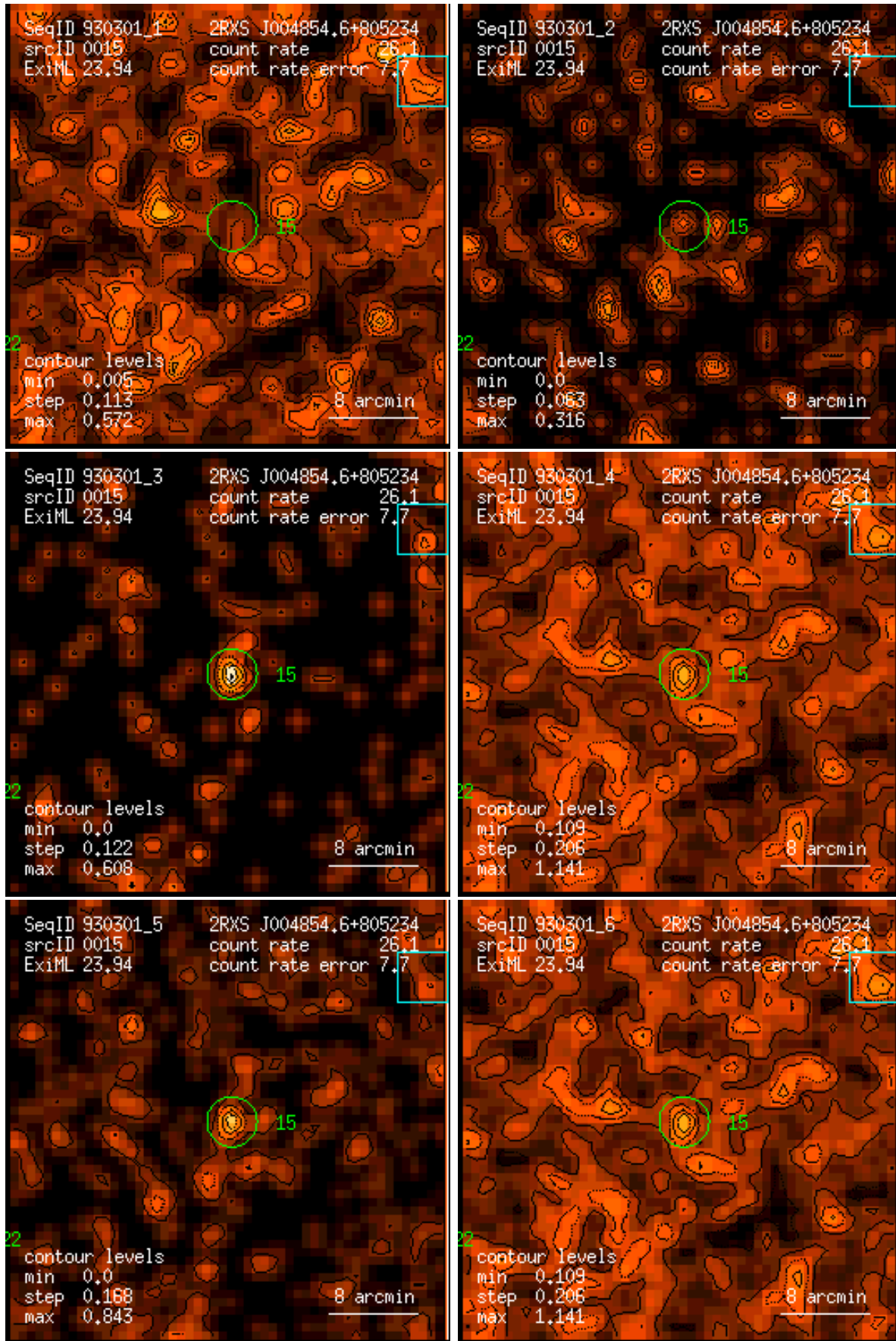
Figure 15: RASS 930301: detection 0015: band rate images, Gaussian filter: (1) PSPC channels 11 – 41, (2) 52 – 90, (3) 91 – 201, (4) 11 – 235, (5) 52 – 201, (6) 11 – 201. Broad band rates in counts/ks. Band rate contour levels in counts/ks/arcmin 2 .
