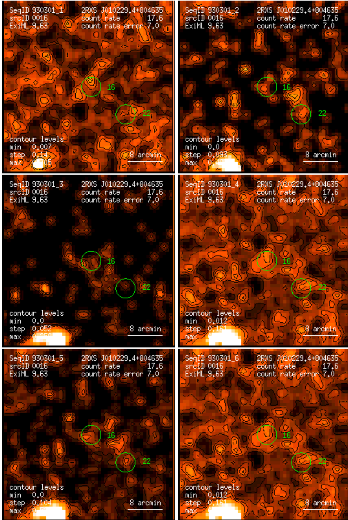
Figure 16: RASS 930301: detection 0016: band rate images, Gaussian filter: (1) PSPC channels 11 – 41, (2) 52 – 90, (3) 91 – 201, (4) 11 – 235, (5) 52 – 201, (6) 11 – 201. Broad band rates in counts/ks. Band rate contour levels in counts/ks/arcmin 2 .
