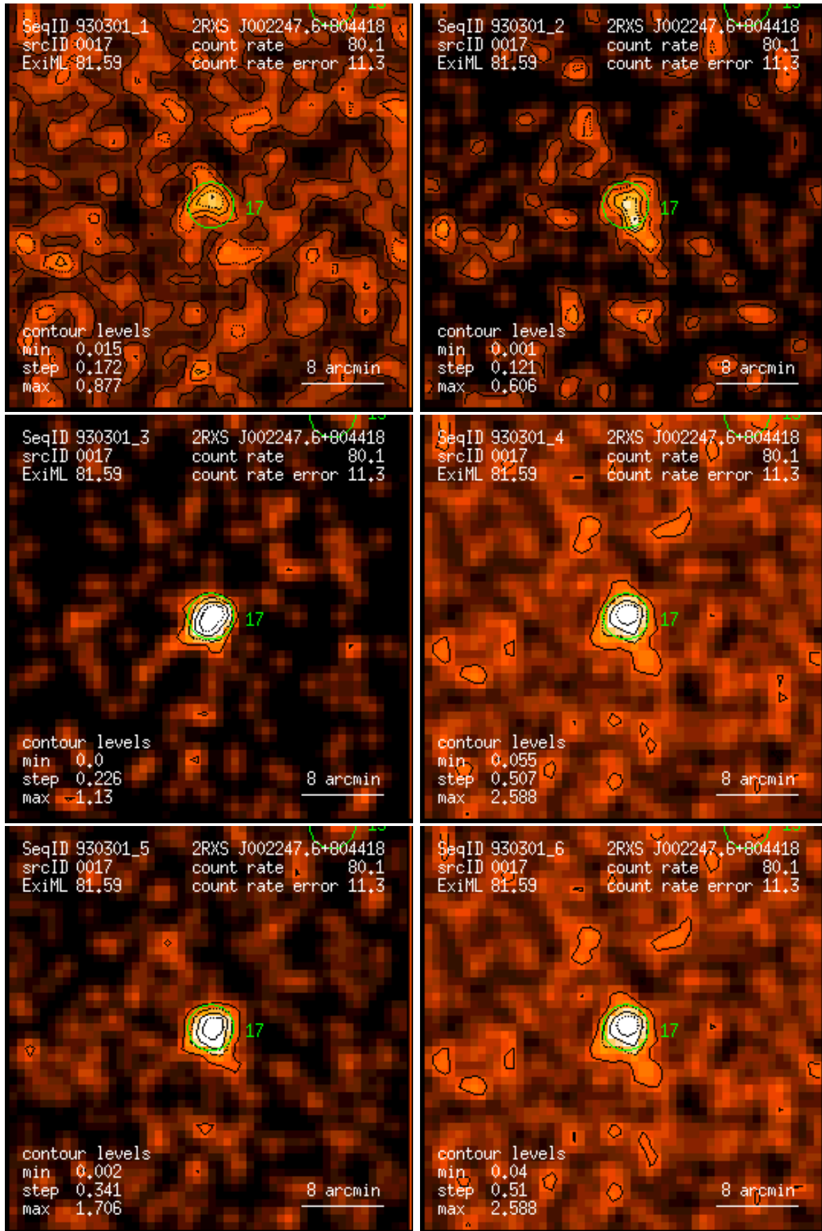
Figure 17: RASS 930301: detection 0017: band rate images, Gaussian filter: (1) PSPC channels 11 – 41, (2) 52 – 90, (3) 91 – 201, (4) 11 – 235, (5) 52 – 201, (6) 11 – 201. Broad band rates in counts/ks. Band rate contour levels in counts/ks/arcmin 2 .
