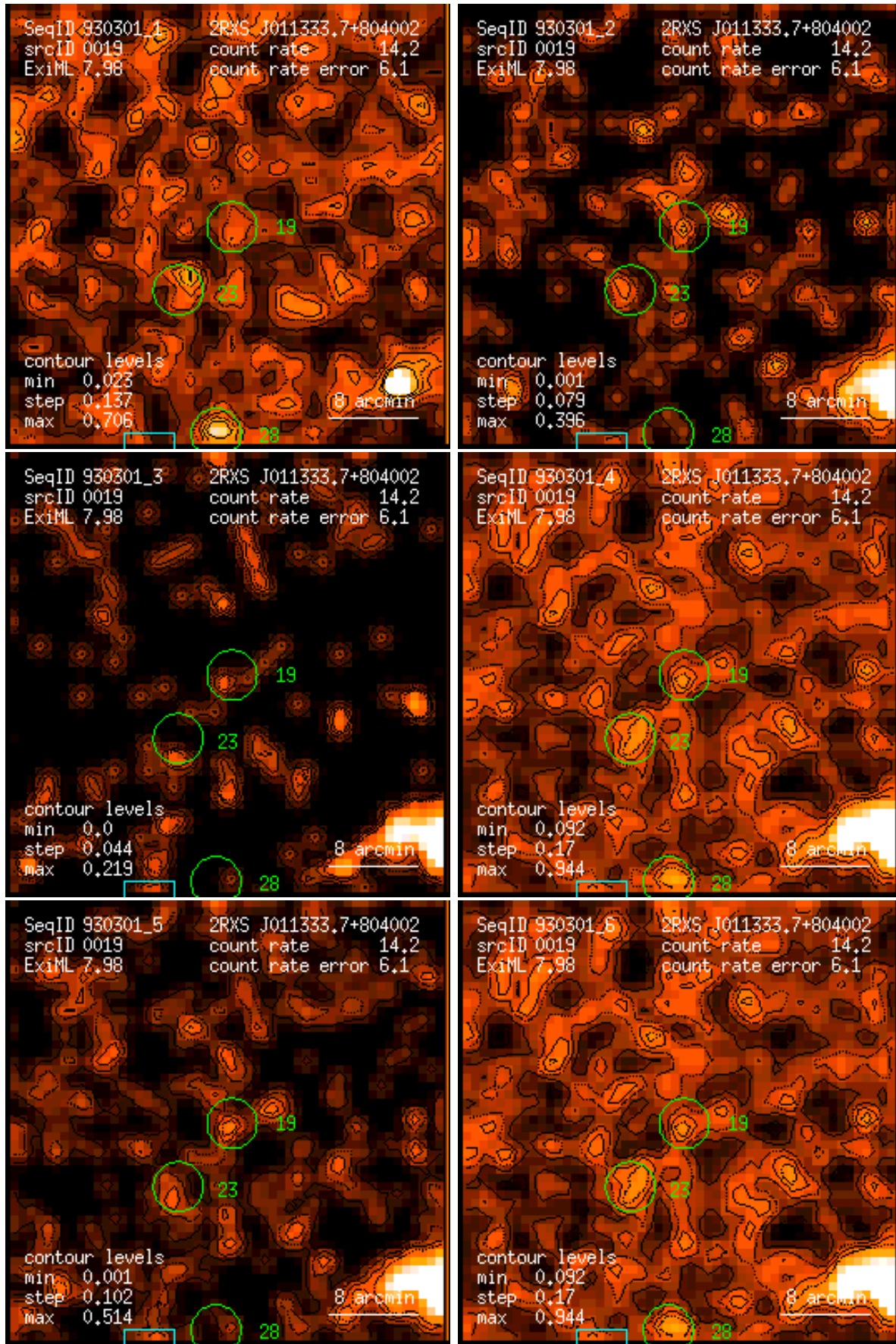
Figure 19: RASS 930301: detection 0019: band rate images, Gaussian filter: (1) PSPC channels 11 – 41, (2) 52 – 90, (3) 91 – 201, (4) 11 – 235, (5) 52 – 201, (6) 11 – 201. Broad band rates in counts/ks. Band rate contour levels in counts/ks/arcmin 2 .
