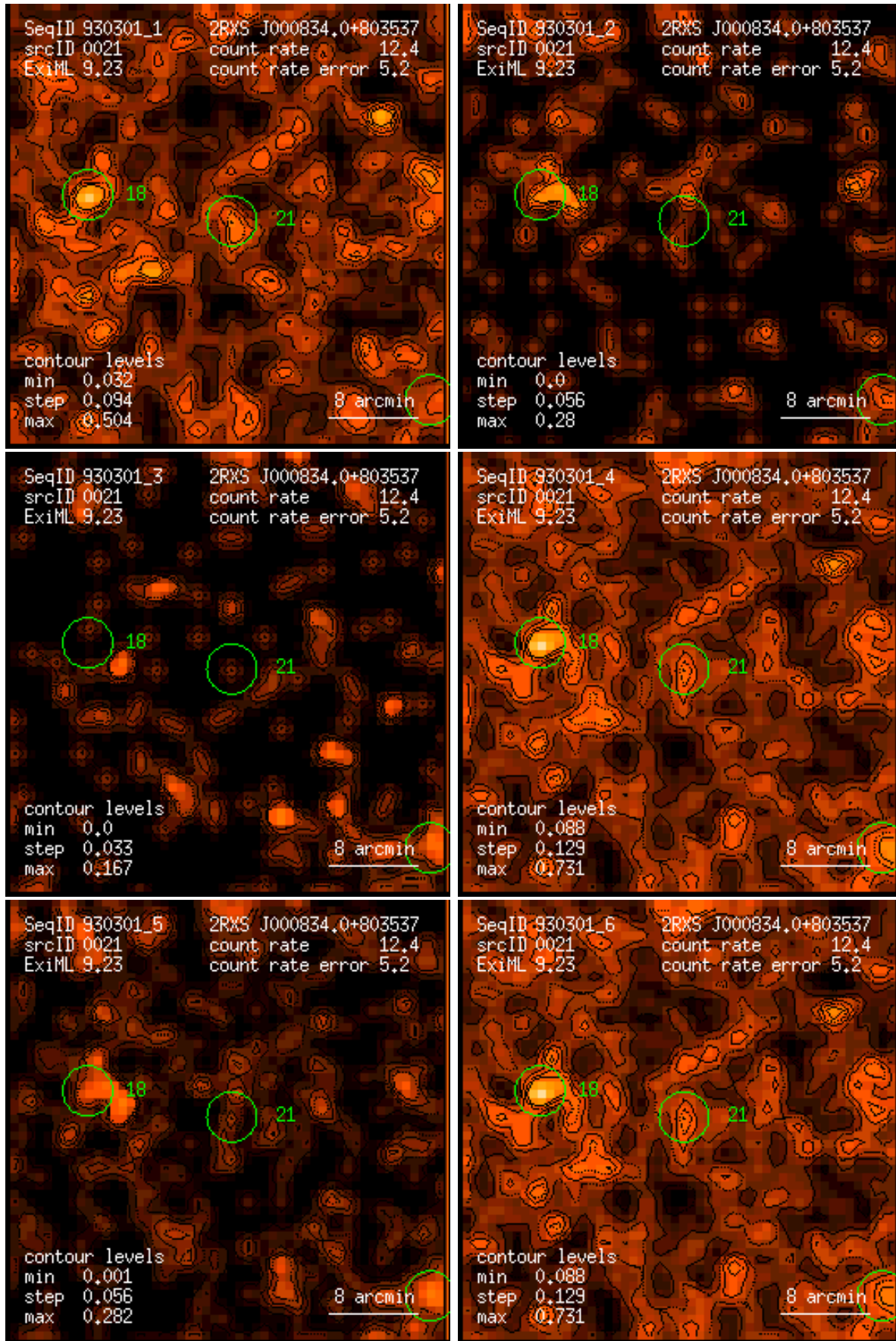
Figure 21: RASS 930301: detection 0021: band rate images, Gaussian filter: (1) PSPC channels 11 – 41, (2) 52 – 90, (3) 91 – 201, (4) 11 – 235, (5) 52 – 201, (6) 11 – 201. Broad band rates in counts/ks. Band rate contour levels in counts/ks/arcmin 2 .
