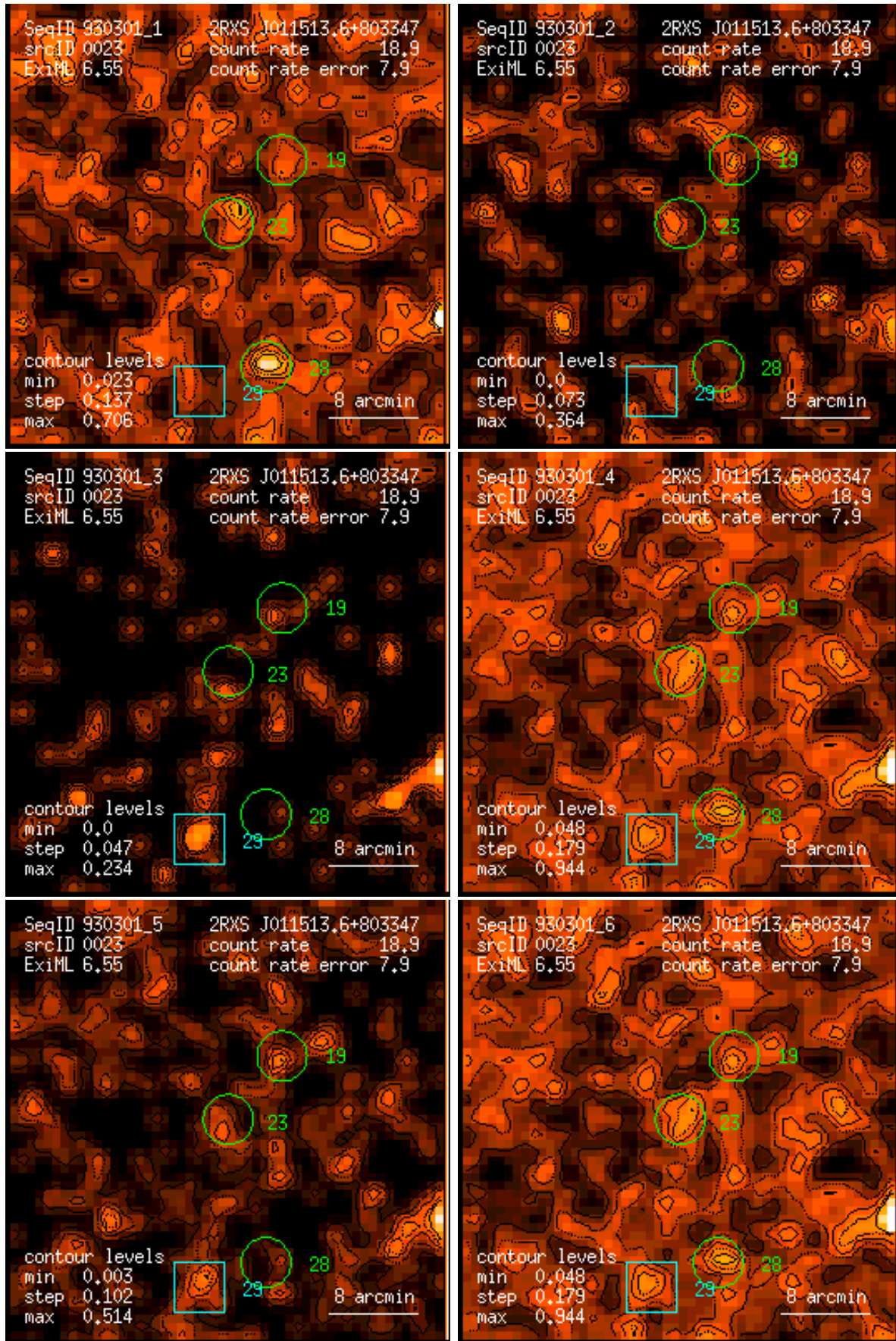
Figure 23: RASS 930301: detection 0023: band rate images, Gaussian filter: (1) PSPC channels 11 – 41, (2) 52 – 90, (3) 91 – 201, (4) 11 – 235, (5) 52 – 201, (6) 11 – 201. Broad band rates in counts/ks. Band rate contour levels in counts/ks/arcmin 2 .
