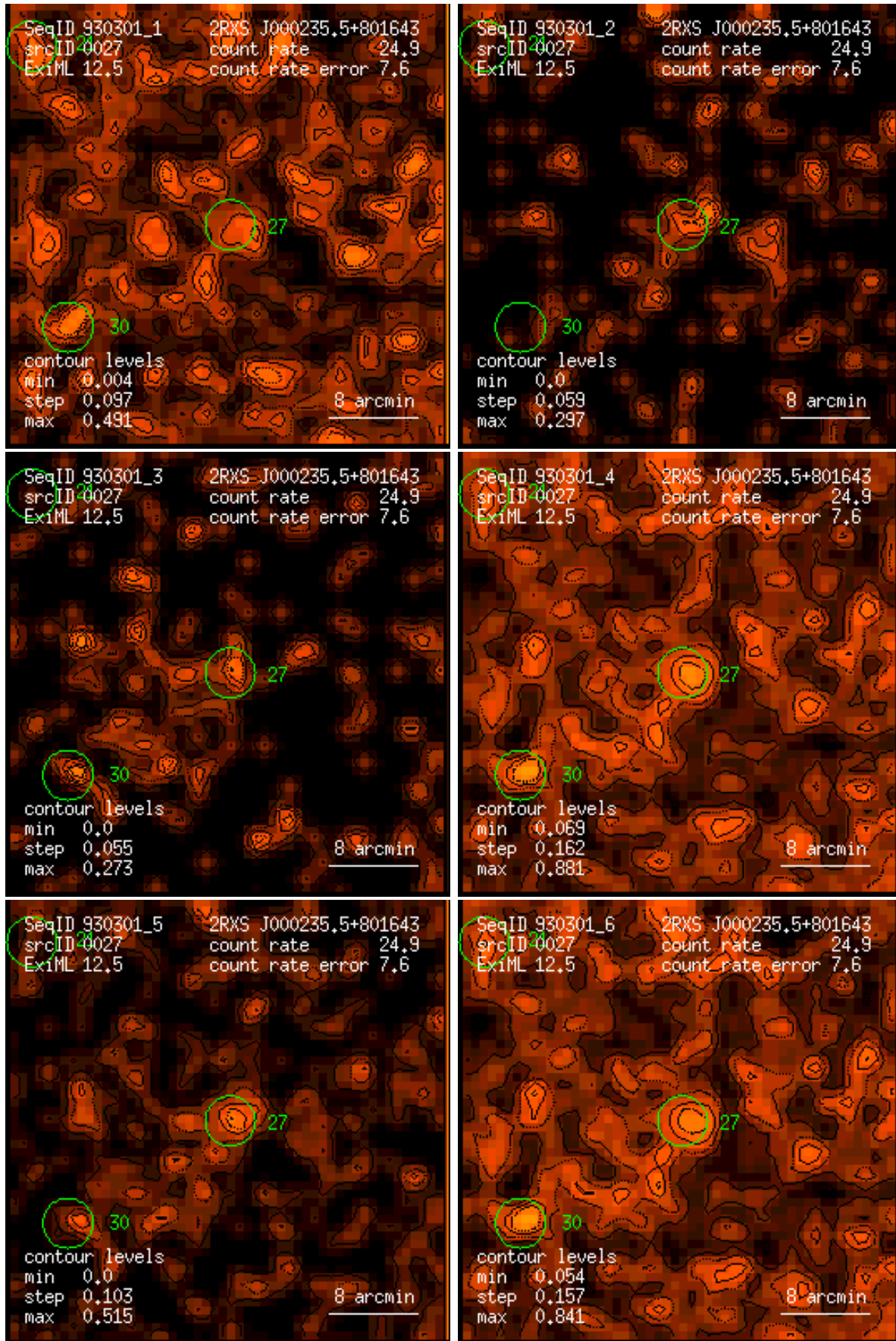
Figure 27: RASS 930301: detection 0027: band rate images, Gaussian filter: (1) PSPC channels 11 – 41, (2) 52 – 90, (3) 91 – 201, (4) 11 – 235, (5) 52 – 201, (6) 11 – 201. Broad band rates in counts/ks. Band rate contour levels in counts/ks/arcmin 2 .
