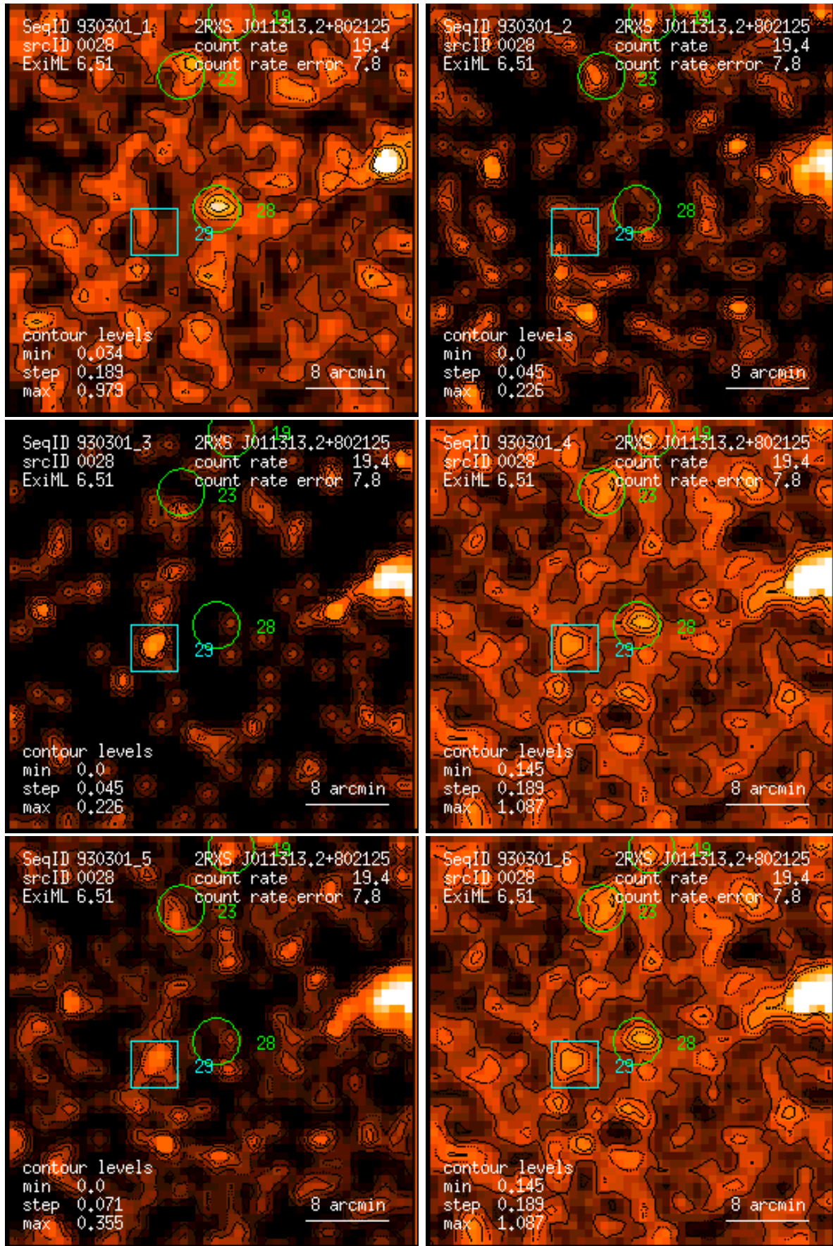
Figure 28: RASS 930301: detection 0028: band rate images, Gaussian filter: (1) PSPC channels 11 – 41, (2) 52 – 90, (3) 91 – 201, (4) 11 – 235, (5) 52 – 201, (6) 11 – 201. Broad band rates in counts/ks. Band rate contour levels in counts/ks/arcmin 2 .
