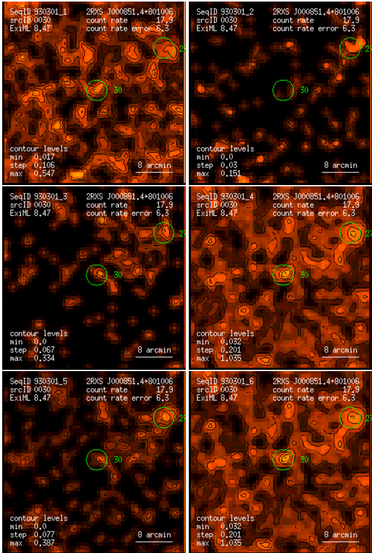
Figure 30: RASS 930301: detection 0030: band rate images, Gaussian filter: (1) PSPC channels 11 – 41, (2) 52 – 90, (3) 91 – 201, (4) 11 – 235, (5) 52 – 201, (6) 11 – 201. Broad band rates in counts/ks. Band rate contour levels in counts/ks/arcmin 2 .
