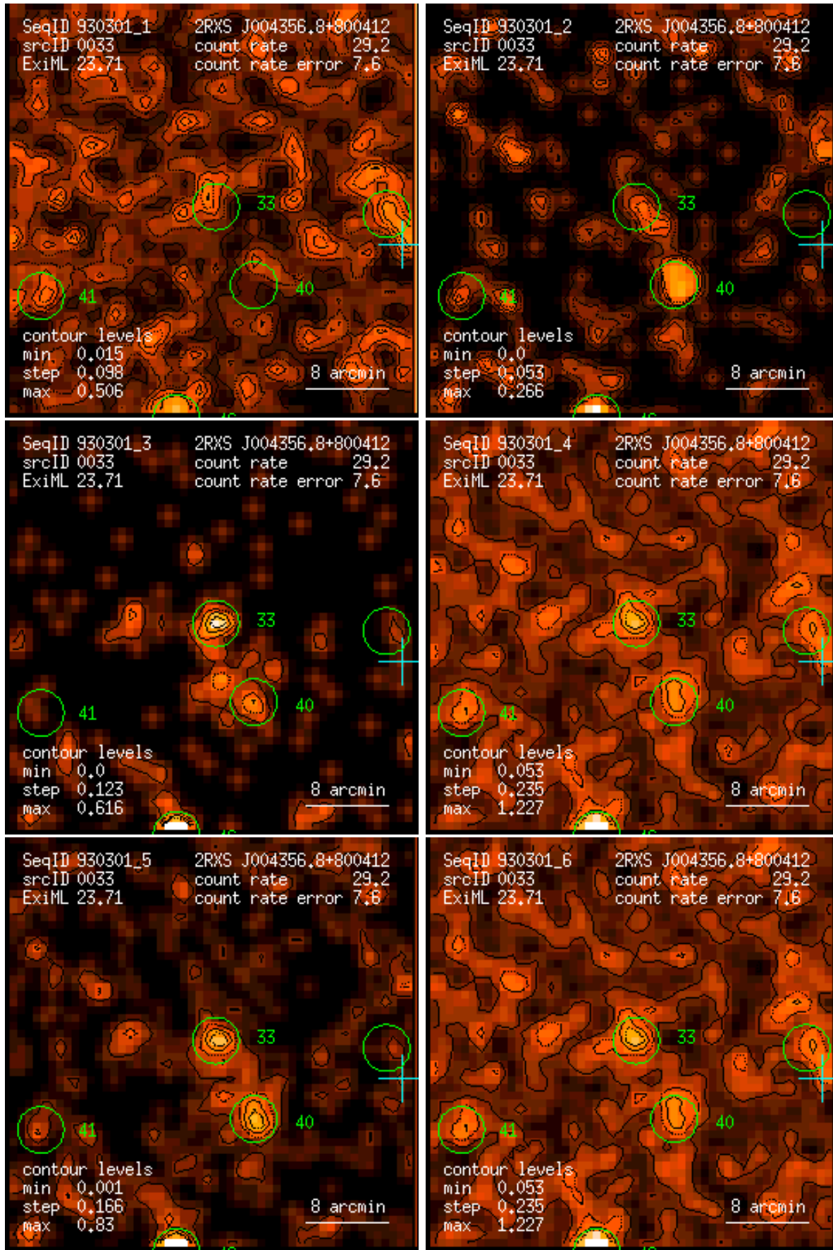
Figure 33: RASS 930301: detection 0033: band rate images, Gaussian filter: (1) PSPC channels 11 – 41, (2) 52 – 90, (3) 91 – 201, (4) 11 – 235, (5) 52 – 201, (6) 11 – 201. Broad band rates in counts/ks. Band rate contour levels in counts/ks/arcmin 2 .
