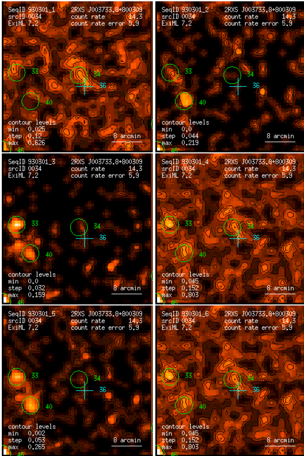
Figure 34: RASS 930301: detection 0034: band rate images, Gaussian filter: (1) PSPC channels 11 – 41, (2) 52 – 90, (3) 91 – 201, (4) 11 – 235, (5) 52 – 201, (6) 11 – 201. Broad band rates in counts/ks. Band rate contour levels in counts/ks/arcmin 2 .
