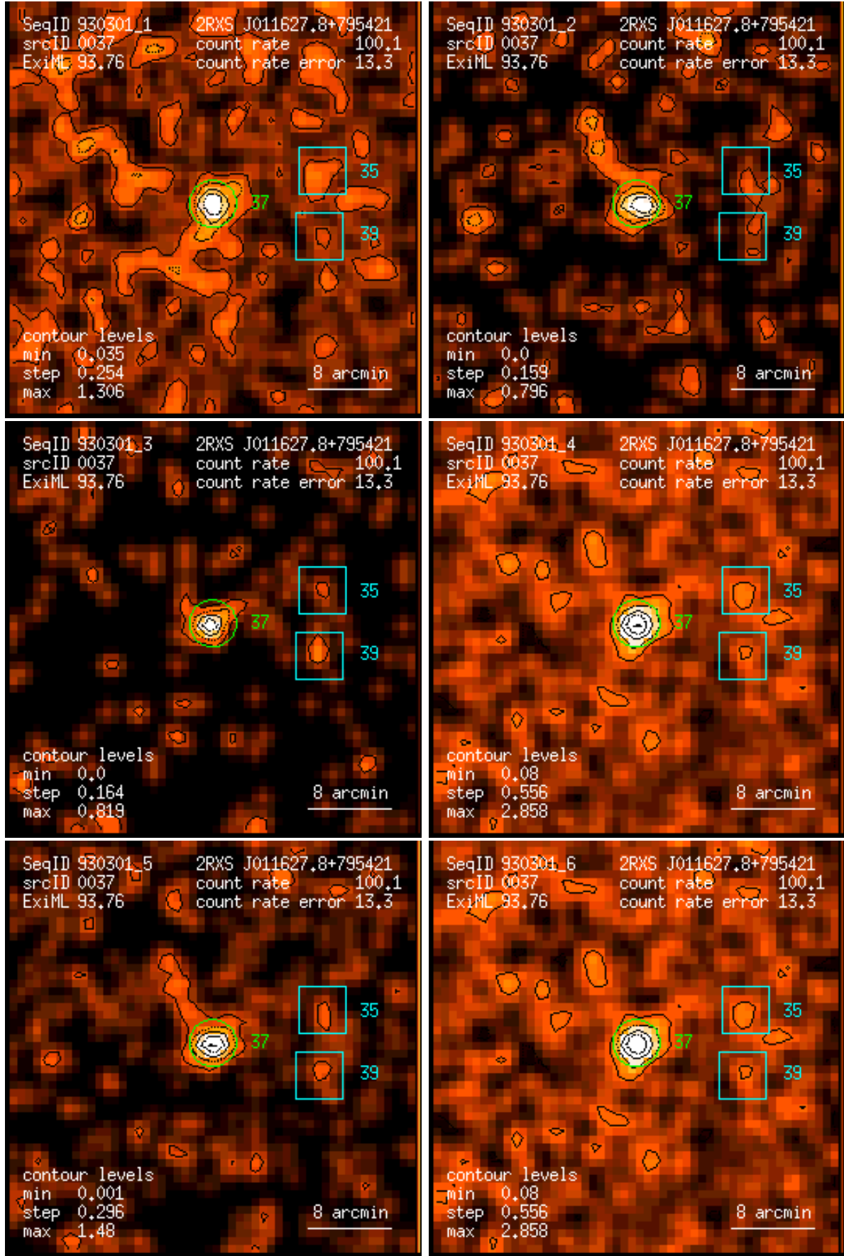
Figure 37: RASS 930301: detection 0037: band rate images, Gaussian filter: (1) PSPC channels 11 – 41, (2) 52 – 90, (3) 91 – 201, (4) 11 – 235, (5) 52 – 201, (6) 11 – 201. Broad band rates in counts/ks. Band rate contour levels in counts/ks/arcmin 2 .
