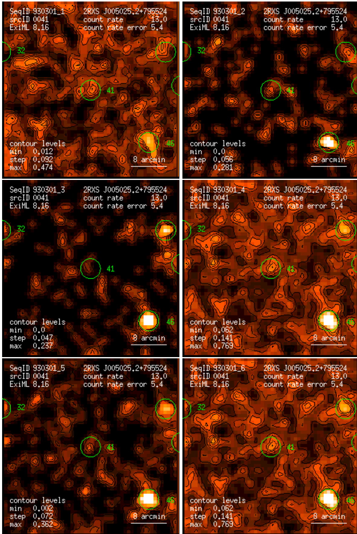
Figure 41: RASS 930301: detection 0041: band rate images, Gaussian filter: (1) PSPC channels 11 – 41, (2) 52 – 90, (3) 91 – 201, (4) 11 – 235, (5) 52 – 201, (6) 11 – 201. Broad band rates in counts/ks. Band rate contour levels in counts/ks/arcmin 2 .
