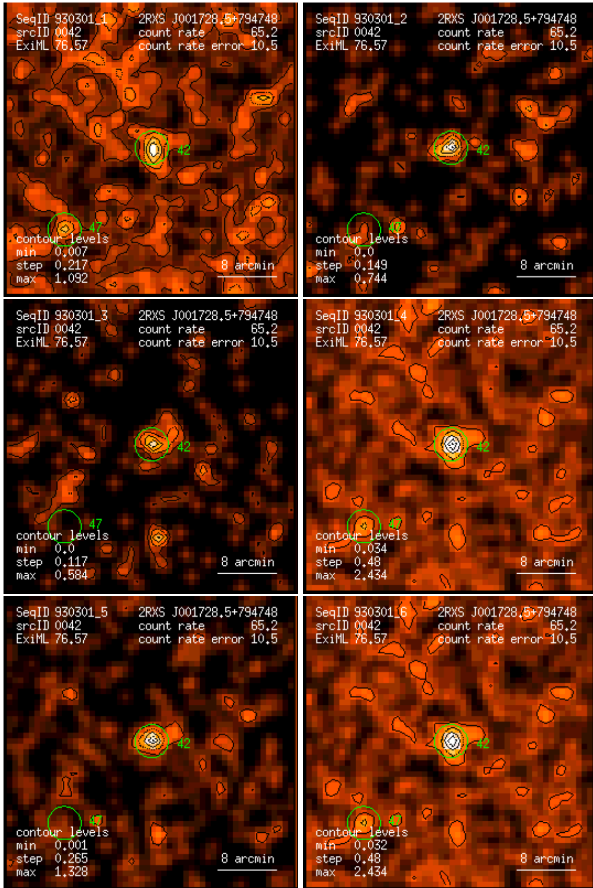
Figure 42: RASS 930301: detection 0042: band rate images, Gaussian filter: (1) PSPC channels 11 – 41, (2) 52 – 90, (3) 91 – 201, (4) 11 – 235, (5) 52 – 201, (6) 11 – 201. Broad band rates in counts/ks. Band rate contour levels in counts/ks/arcmin 2 .
