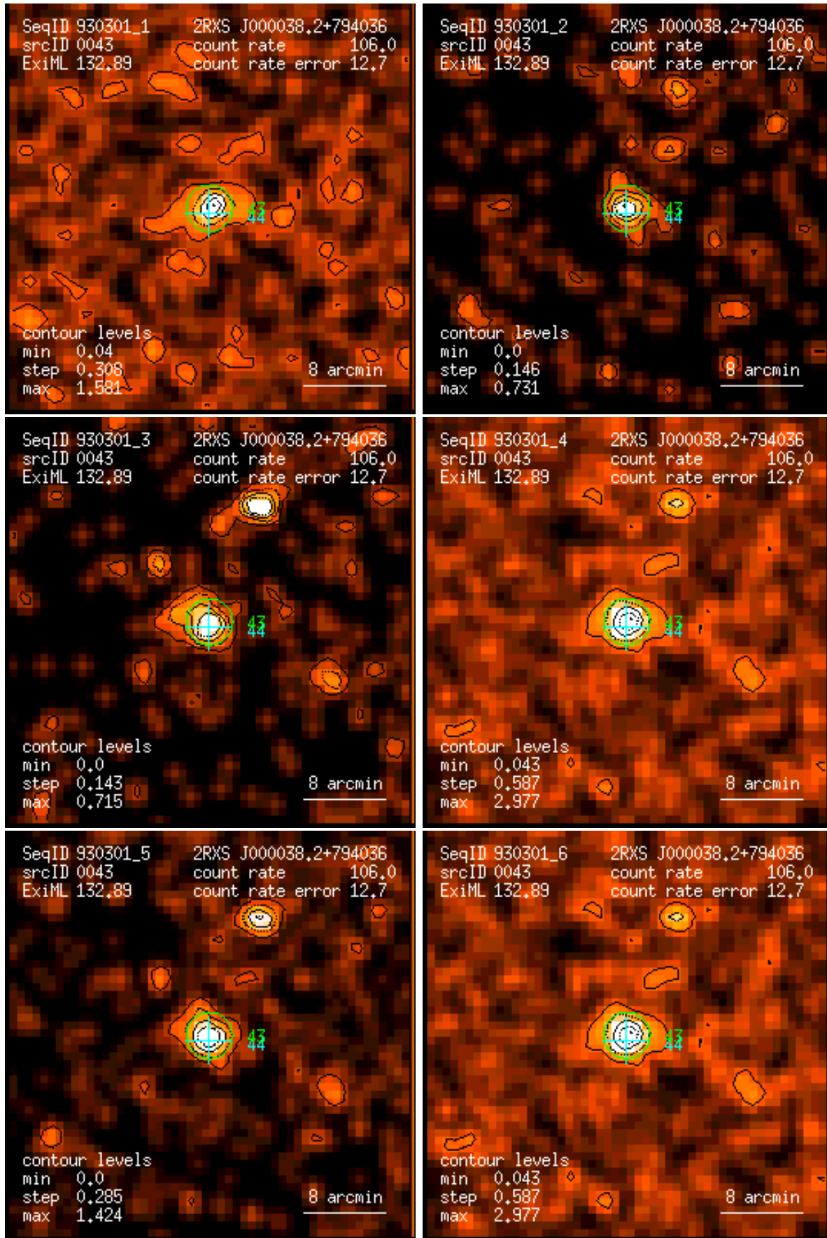
Figure 43: RASS 930301: detection 0043: band rate images, Gaussian filter: (1) PSPC channels 11 – 41, (2) 52 – 90, (3) 91 – 201, (4) 11 – 235, (5) 52 – 201, (6) 11 – 201. Broad band rates in counts/ks. Band rate contour levels in counts/ks/arcmin 2 .
