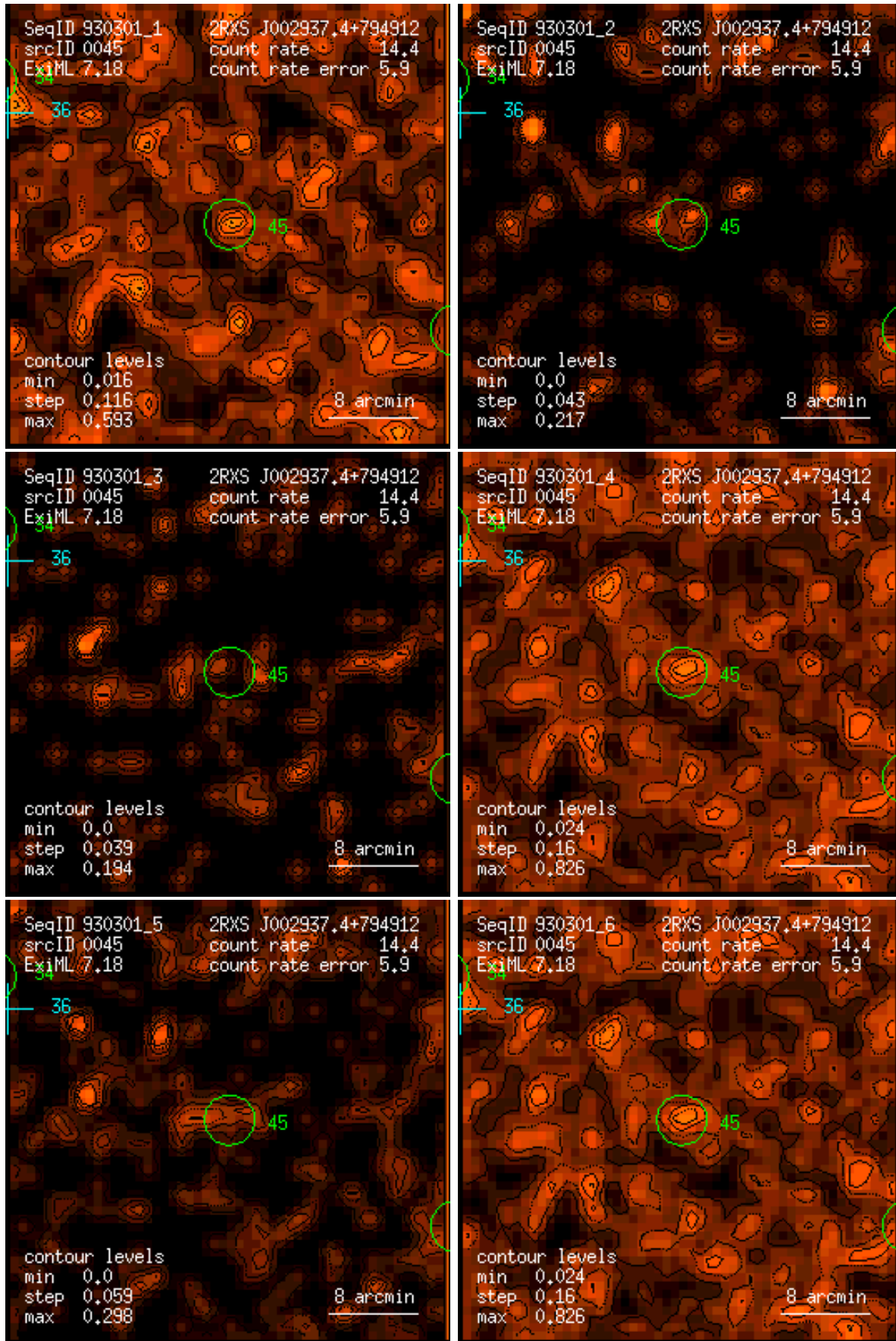
Figure 45: RASS 930301: detection 0045: band rate images, Gaussian filter: (1) PSPC channels 11 – 41, (2) 52 – 90, (3) 91 – 201, (4) 11 – 235, (5) 52 – 201, (6) 11 – 201. Broad band rates in counts/ks. Band rate contour levels in counts/ks/arcmin 2 .
