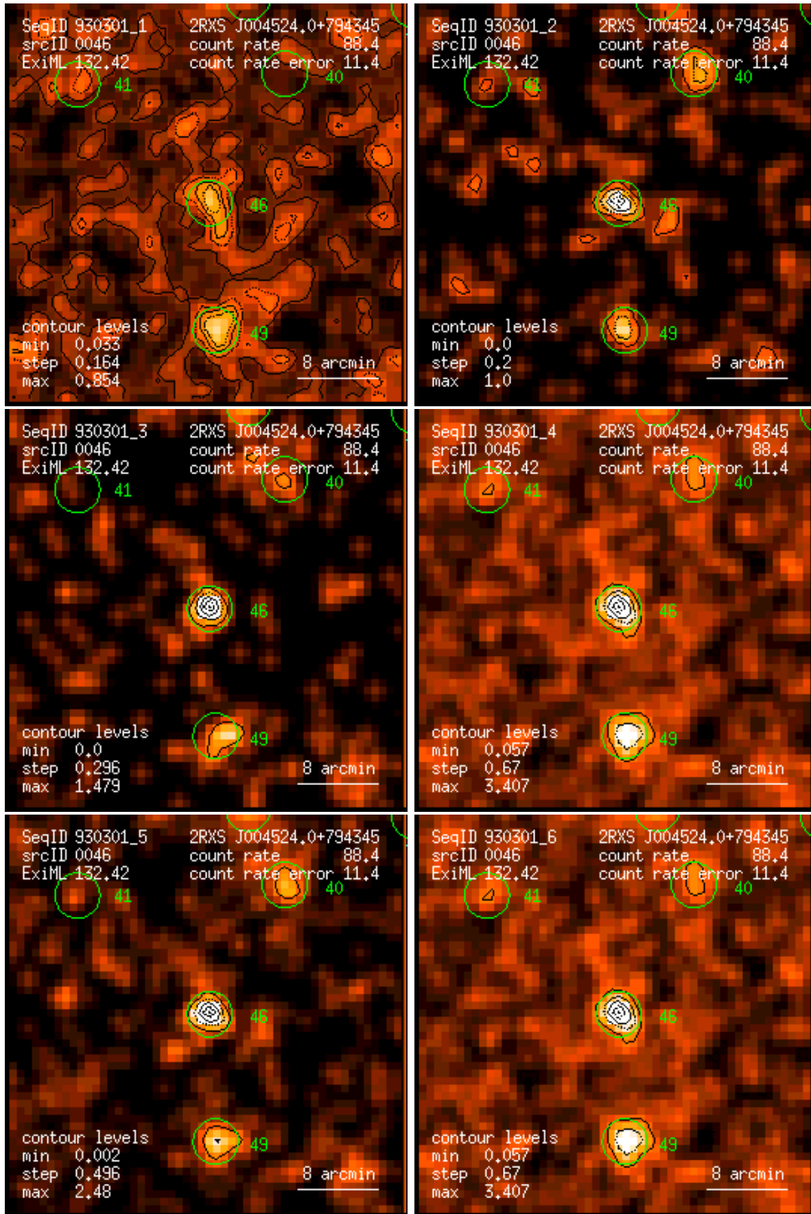
Figure 46: RASS 930301: detection 0046: band rate images, Gaussian filter: (1) PSPC channels 11 – 41, (2) 52 – 90, (3) 91 – 201, (4) 11 – 235, (5) 52 – 201, (6) 11 – 201. Broad band rates in counts/ks. Band rate contour levels in counts/ks/arcmin 2 .
