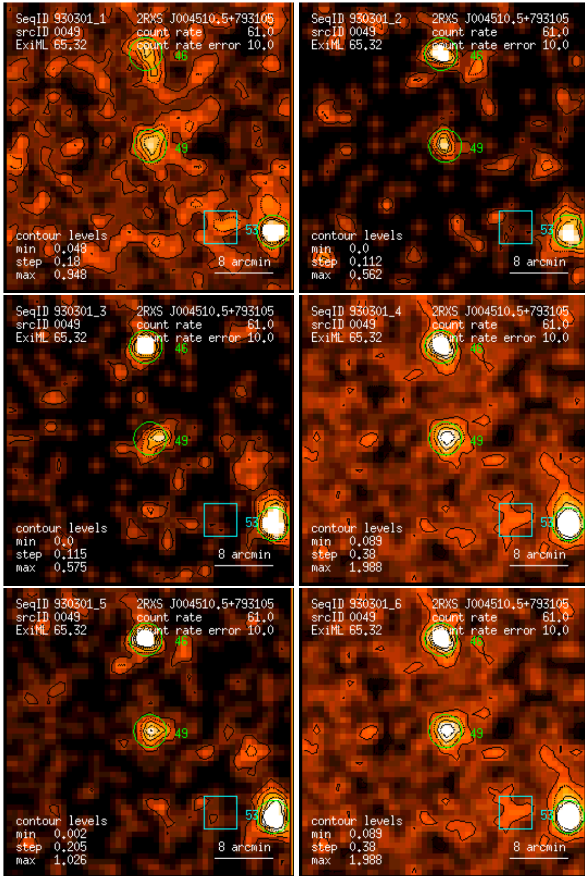
Figure 49: RASS 930301: detection 0049: band rate images, Gaussian filter: (1) PSPC channels 11 – 41, (2) 52 – 90, (3) 91 – 201, (4) 11 – 235, (5) 52 – 201, (6) 11 – 201. Broad band rates in counts/ks. Band rate contour levels in counts/ks/arcmin 2 .
