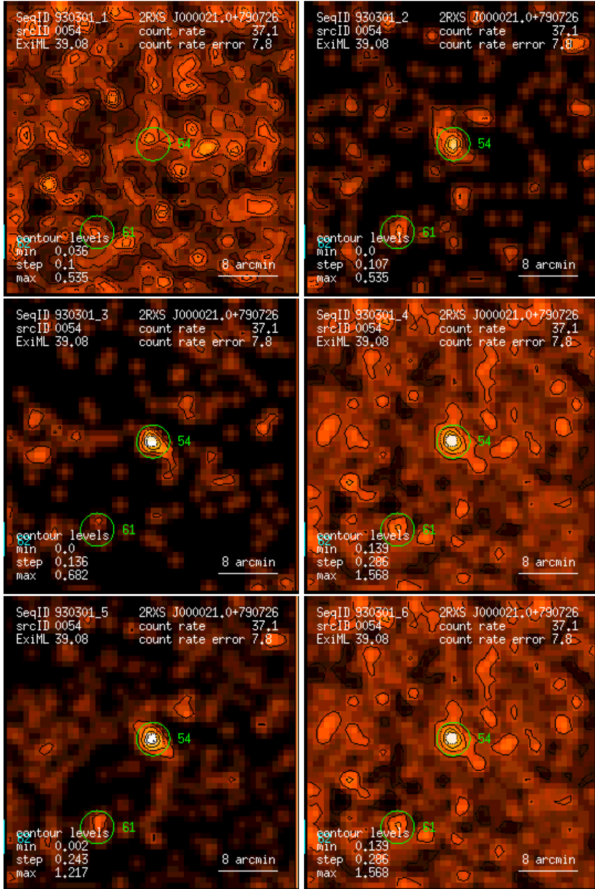
Figure 54: RASS 930301: detection 0054: band rate images, Gaussian filter: (1) PSPC channels 11 – 41, (2) 52 – 90, (3) 91 – 201, (4) 11 – 235, (5) 52 – 201, (6) 11 – 201. Broad band rates in counts/ks. Band rate contour levels in counts/ks/arcmin 2 .
