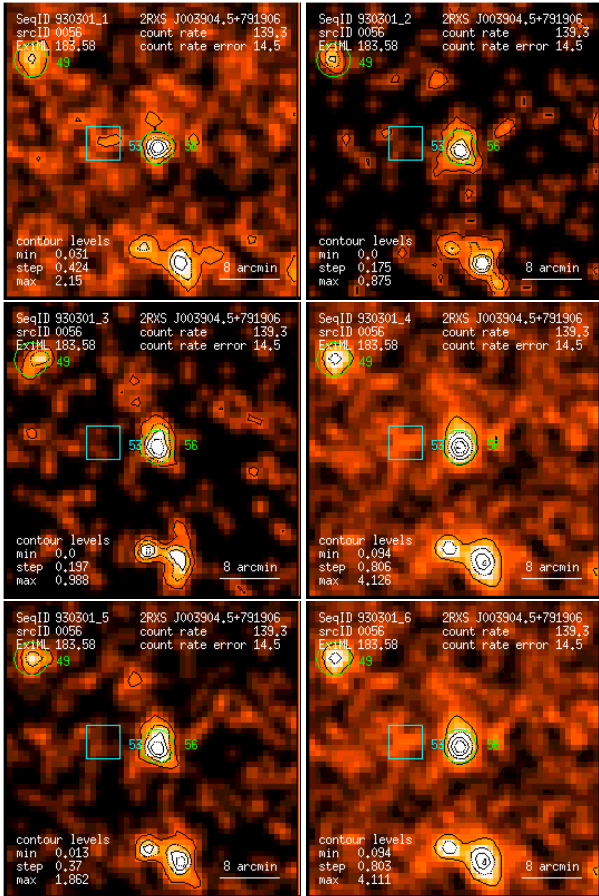
Figure 56: RASS 930301: detection 0056: band rate images, Gaussian filter: (1) PSPC channels 11 – 41, (2) 52 – 90, (3) 91 – 201, (4) 11 – 235, (5) 52 – 201, (6) 11 – 201. Broad band rates in counts/ks. Band rate contour levels in counts/ks/arcmin 2 .
