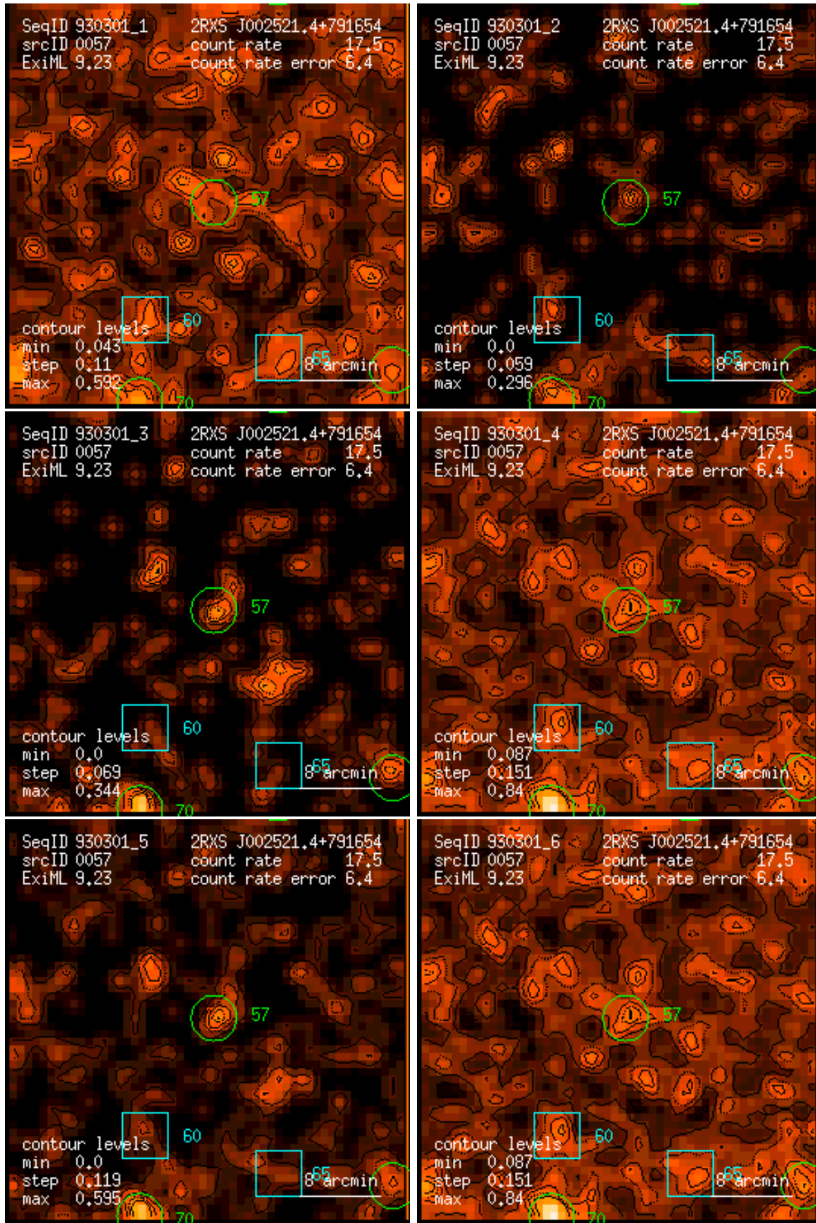
Figure 57: RASS 930301: detection 0057: band rate images, Gaussian filter: (1) PSPC channels 11 – 41, (2) 52 – 90, (3) 91 – 201, (4) 11 – 235, (5) 52 – 201, (6) 11 – 201. Broad band rates in counts/ks. Band rate contour levels in counts/ks/arcmin 2 .
