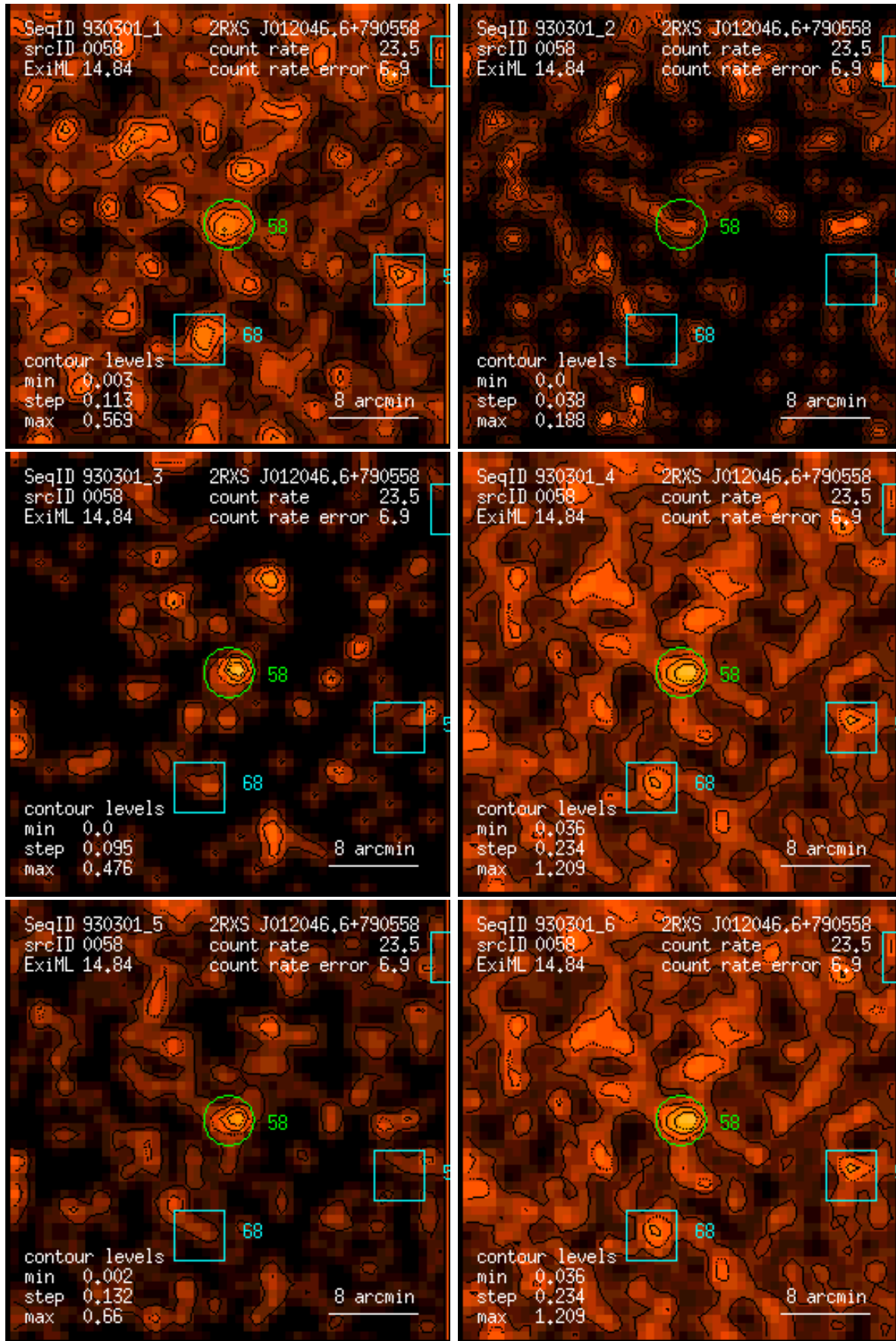
Figure 58: RASS 930301: detection 0058: band rate images, Gaussian filter: (1) PSPC channels 11 – 41, (2) 52 – 90, (3) 91 – 201, (4) 11 – 235, (5) 52 – 201, (6) 11 – 201. Broad band rates in counts/ks. Band rate contour levels in counts/ks/arcmin 2 .
