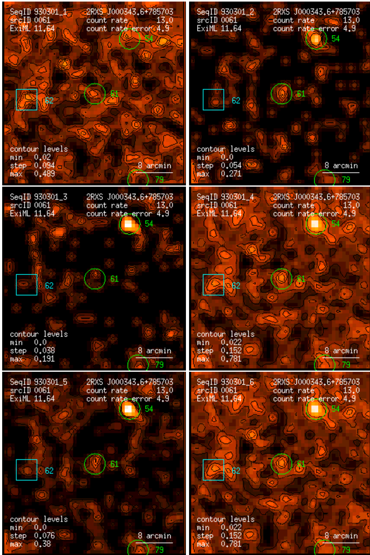
Figure 61: RASS 930301: detection 0061: band rate images, Gaussian filter: (1) PSPC channels 11 – 41, (2) 52 – 90, (3) 91 – 201, (4) 11 – 235, (5) 52 – 201, (6) 11 – 201. Broad band rates in counts/ks. Band rate contour levels in counts/ks/arcmin 2 .
