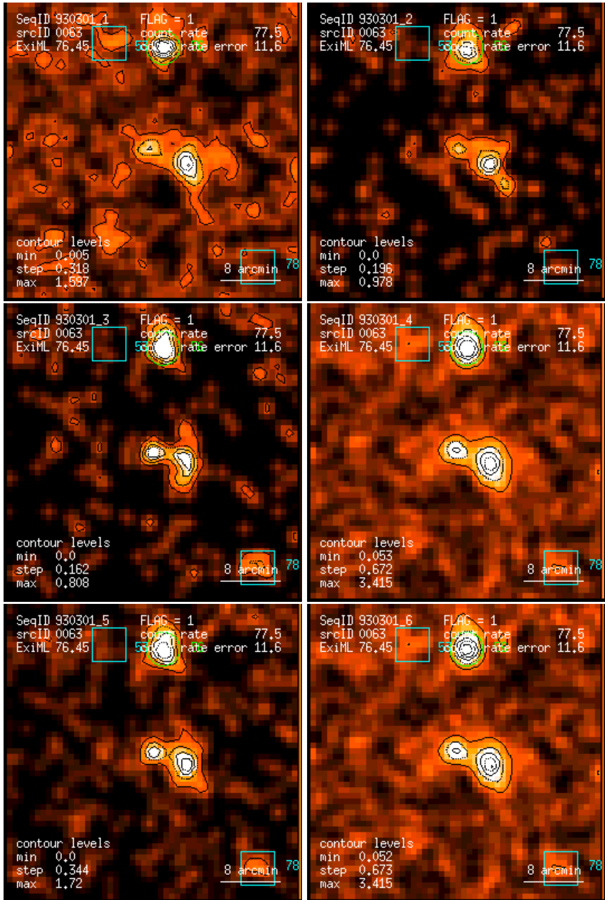
Figure 63: RASS 930301: detection 0063: band rate images, Gaussian filter: (1) PSPC channels 11 – 41, (2) 52 – 90, (3) 91 – 201, (4) 11 – 235, (5) 52 – 201, (6) 11 – 201. Broad band rates in counts/ks. Band rate contour levels in counts/ks/arcmin 2 .
