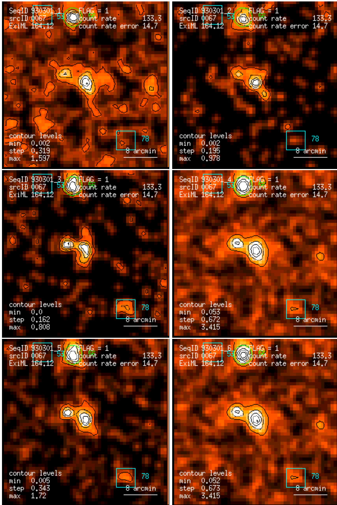
Figure 67: RASS 930301: detection 0067: band rate images, Gaussian filter: (1) PSPC channels 11 – 41, (2) 52 – 90, (3) 91 – 201, (4) 11 – 235, (5) 52 – 201, (6) 11 – 201. Broad band rates in counts/ks. Band rate contour levels in counts/ks/arcmin 2 .
