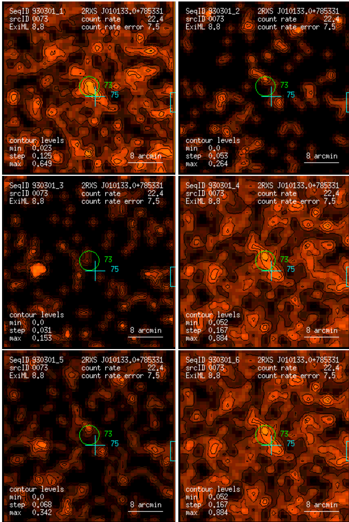
Figure 73: RASS 930301: detection 0073: band rate images, Gaussian filter: (1) PSPC channels 11 – 41, (2) 52 – 90, (3) 91 – 201, (4) 11 – 235, (5) 52 – 201, (6) 11 – 201. Broad band rates in counts/ks. Band rate contour levels in counts/ks/arcmin 2 .
