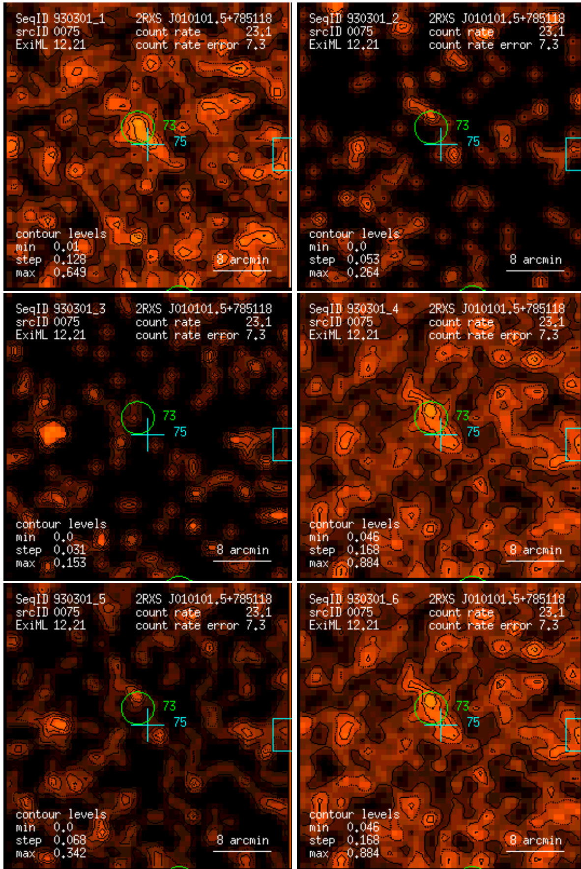
Figure 75: RASS 930301: detection 0075: band rate images, Gaussian filter: (1) PSPC channels 11 – 41, (2) 52 – 90, (3) 91 – 201, (4) 11 – 235, (5) 52 – 201, (6) 11 – 201. Broad band rates in counts/ks. Band rate contour levels in counts/ks/arcmin 2 .
