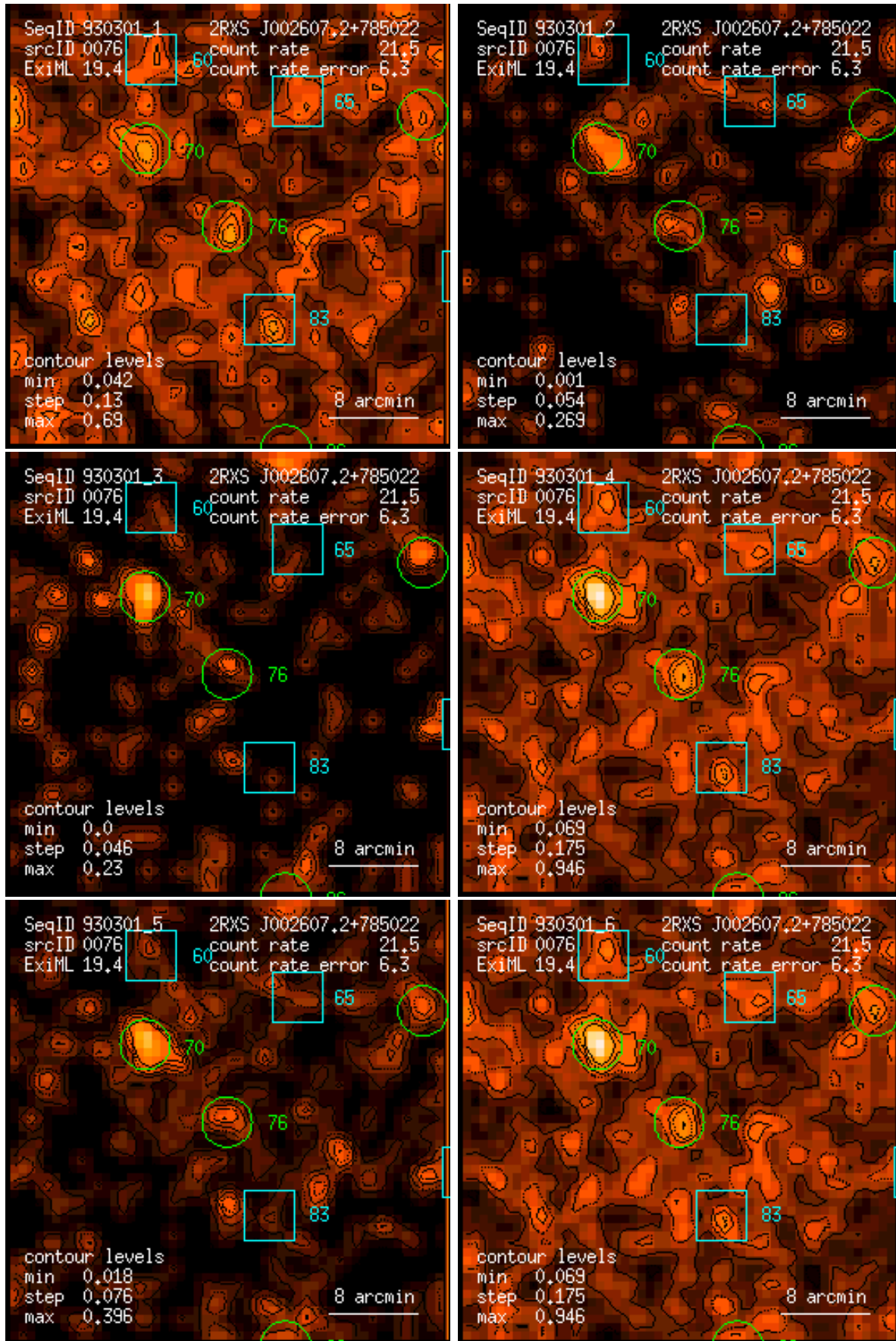
Figure 76: RASS 930301: detection 0076: band rate images, Gaussian filter: (1) PSPC channels 11 – 41, (2) 52 – 90, (3) 91 – 201, (4) 11 – 235, (5) 52 – 201, (6) 11 – 201. Broad band rates in counts/ks. Band rate contour levels in counts/ks/arcmin 2 .
