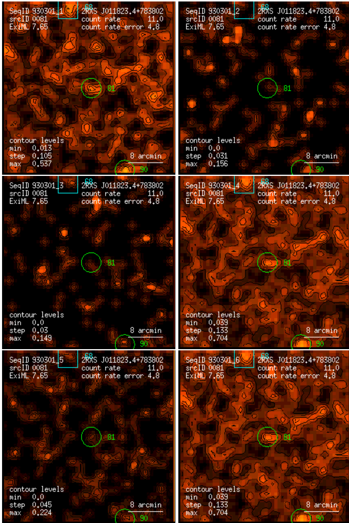
Figure 81: RASS 930301: detection 0081: band rate images, Gaussian filter: (1) PSPC channels 11 – 41, (2) 52 – 90, (3) 91 – 201, (4) 11 – 235, (5) 52 – 201, (6) 11 – 201. Broad band rates in counts/ks. Band rate contour levels in counts/ks/arcmin 2 .
