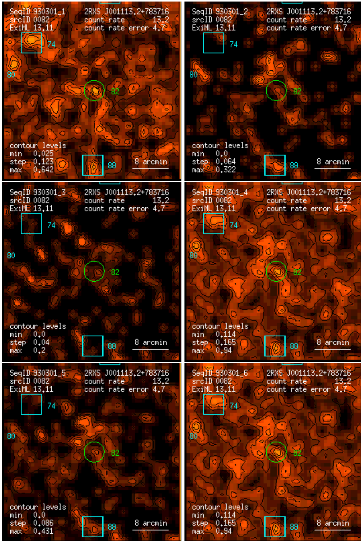
Figure 82: RASS 930301: detection 0082: band rate images, Gaussian filter: (1) PSPC channels 11 – 41, (2) 52 – 90, (3) 91 – 201, (4) 11 – 235, (5) 52 – 201, (6) 11 – 201. Broad band rates in counts/ks. Band rate contour levels in counts/ks/arcmin 2 .
