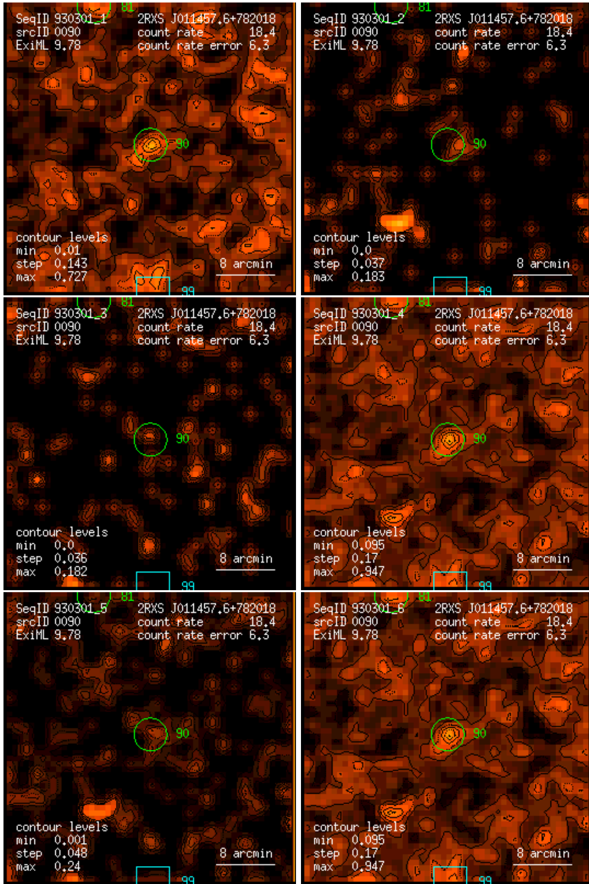
Figure 90: RASS 930301: detection 0090: band rate images, Gaussian filter: (1) PSPC channels 11 – 41, (2) 52 – 90, (3) 91 – 201, (4) 11 – 235, (5) 52 – 201, (6) 11 – 201. Broad band rates in counts/ks. Band rate contour levels in counts/ks/arcmin 2 .
