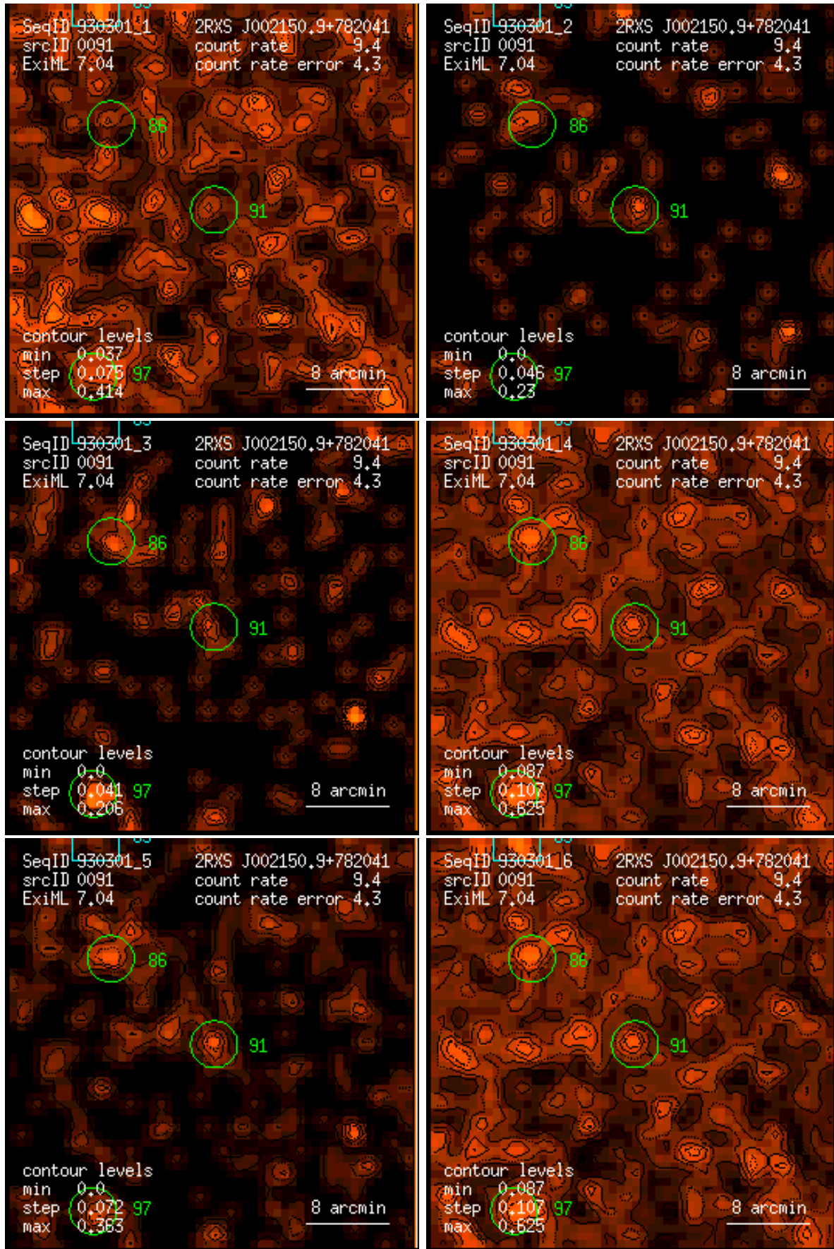
Figure 91: RASS 930301: detection 0091: band rate images, Gaussian filter: (1) PSPC channels 11 – 41, (2) 52 – 90, (3) 91 – 201, (4) 11 – 235, (5) 52 – 201, (6) 11 – 201. Broad band rates in counts/ks. Band rate contour levels in counts/ks/arcmin 2 .
