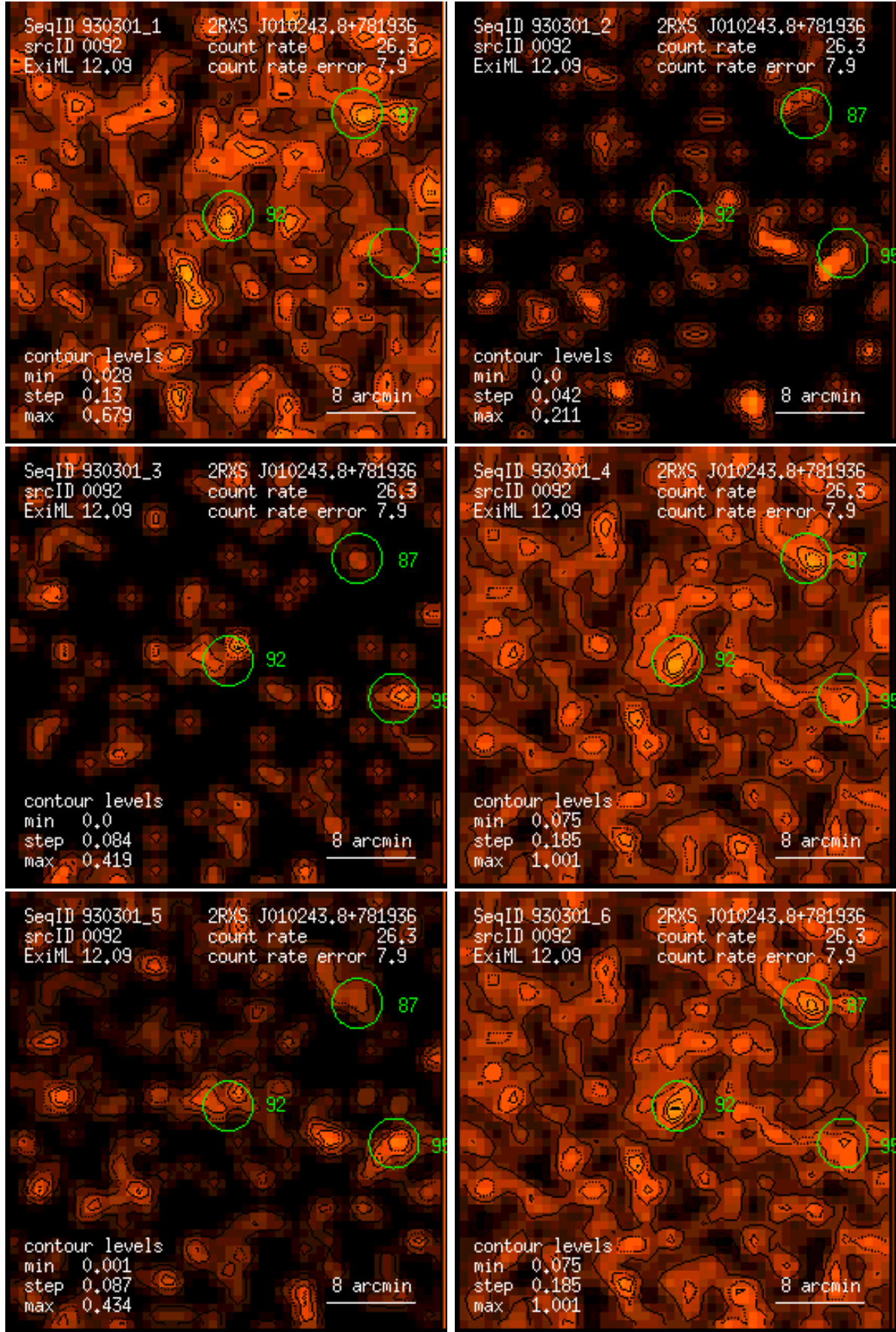
Figure 92: RASS 930301: detection 0092: band rate images, Gaussian filter: (1) PSPC channels 11 – 41, (2) 52 – 90, (3) 91 – 201, (4) 11 – 235, (5) 52 – 201, (6) 11 – 201. Broad band rates in counts/ks. Band rate contour levels in counts/ks/arcmin 2 .
