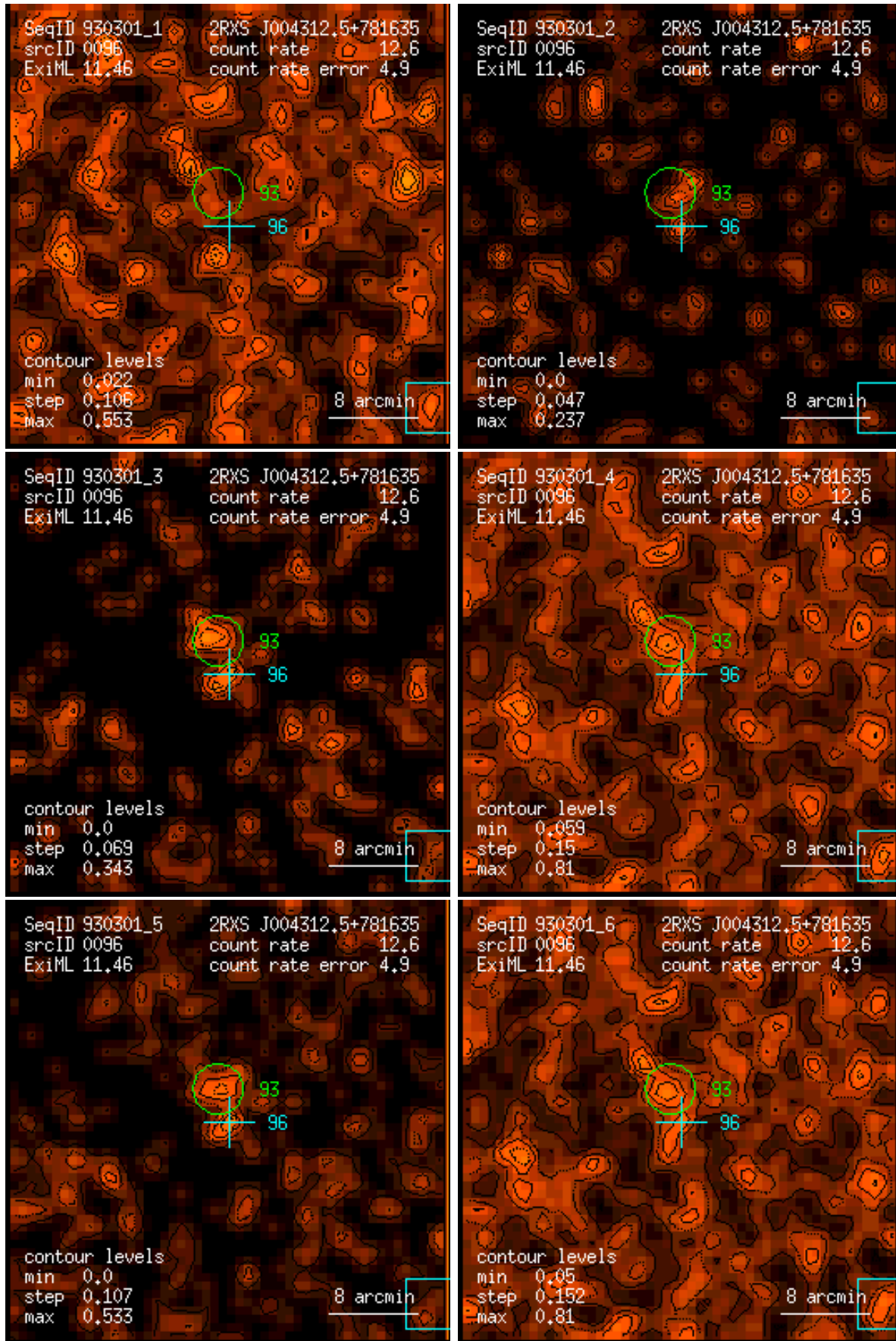
Figure 96: RASS 930301: detection 0096: band rate images, Gaussian filter: (1) PSPC channels 11 – 41, (2) 52 – 90, (3) 91 – 201, (4) 11 – 235, (5) 52 – 201, (6) 11 – 201. Broad band rates in counts/ks. Band rate contour levels in counts/ks/arcmin 2 .
